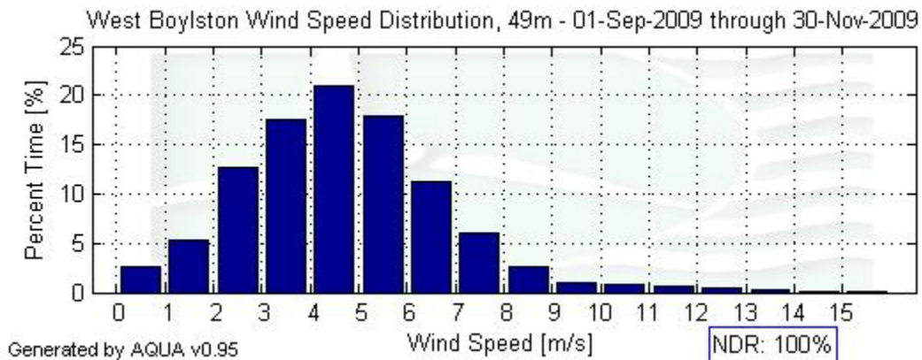
Figure 2 – Wind Speed Distribution, September 1 – November 30, 2009
