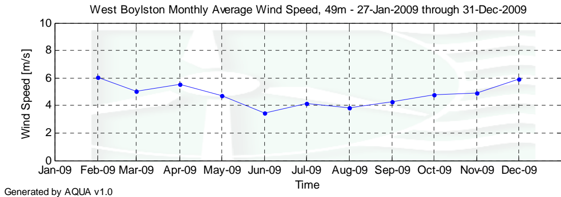
Figure 3 - Monthly Average Wind Speed, February 2009 – December 2009
