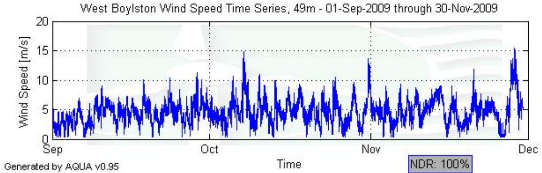
Figure 1 – Wind Speed Time Series, September 1 – November 30, 2009
