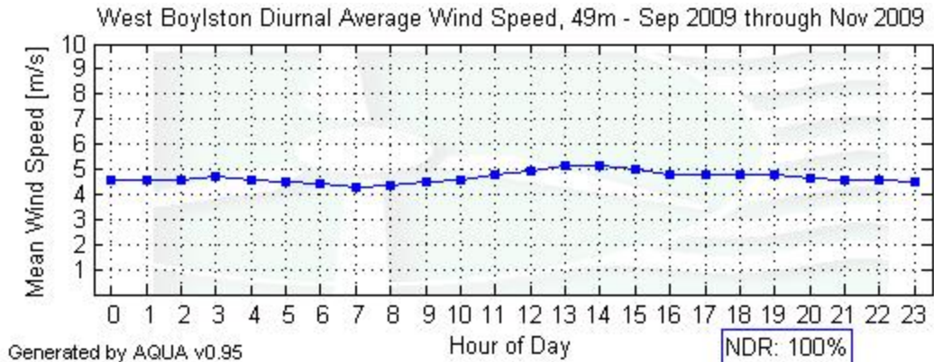
Figure 4 - Diurnal Average Wind Speeds, September 1 – November 30, 2009
