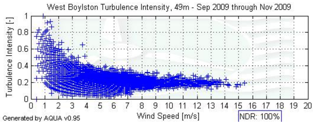
Figure 5 - Turbulence Intensity vs. Wind Speed, September 1 – November 30, 2009
