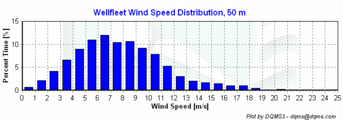
Figure 3 - Wind Speed Distribution, March 1, 2007 – May 31, 2007
