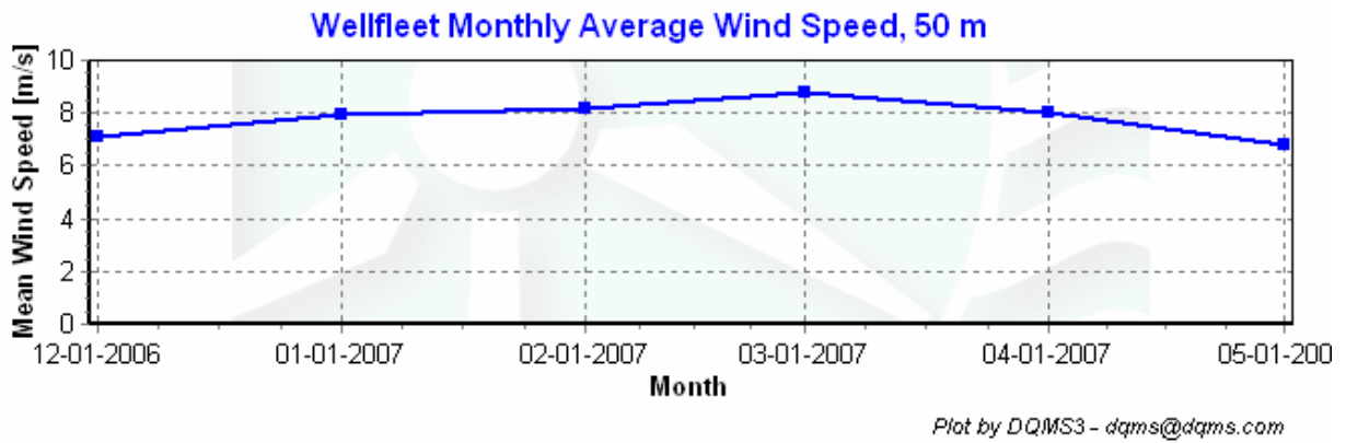
Figure 4 – Monthly Average Wind Speed, December 1, 2006 – May 31, 2007
