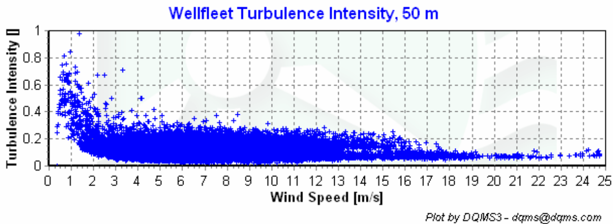
Figure 6 – Turbulence Intensity, March 1, 2007 – May 31, 2007
