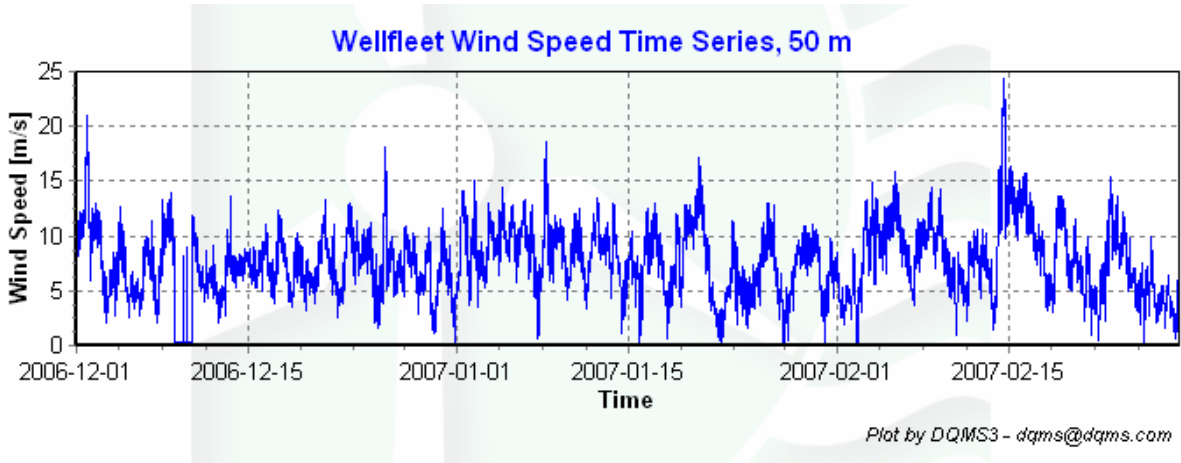
Figure 2 - Wind Speed Time Series, December 1, 2006 – February 28, 2007
