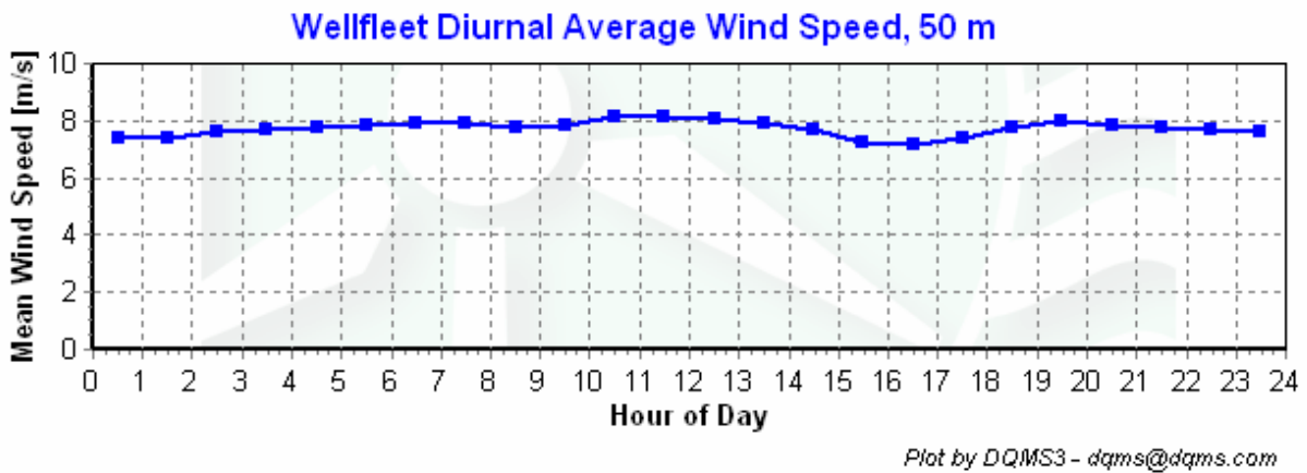
Figure 5 - Diurnal Average Wind Speed, December 1, 2006 – February 28, 2007
