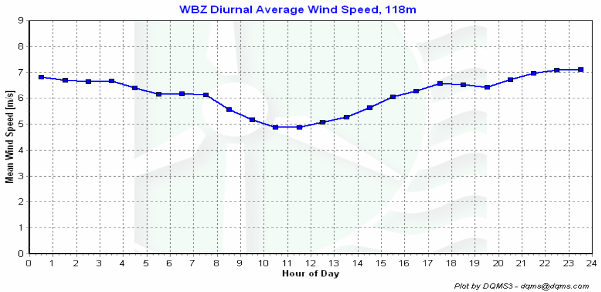
Figure 4 - WBZ Tower Diurnal Average Wind Speed for March 22 to May 31
