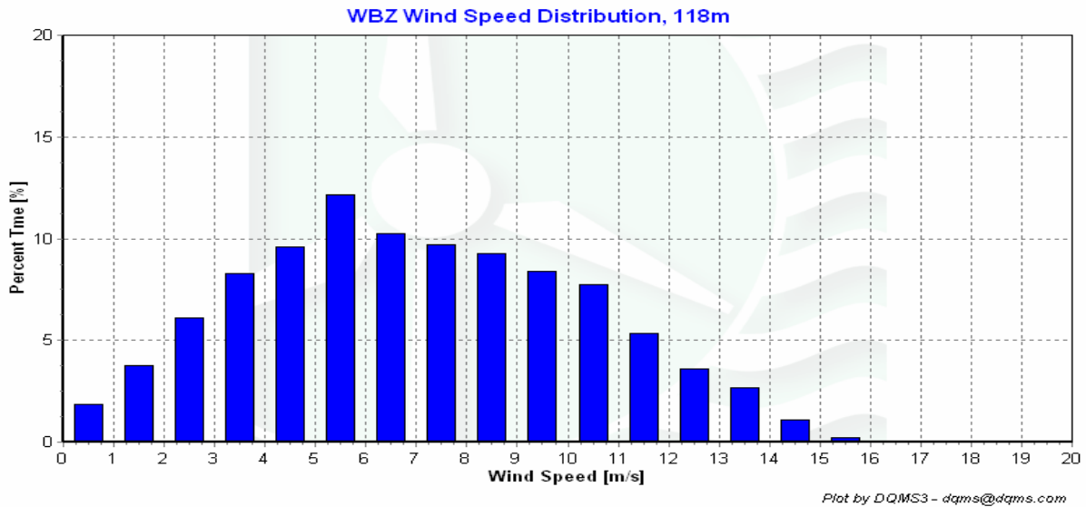
Figure 3 - WBZ Tower Wind Speed Distribution for March 22 to May 31
