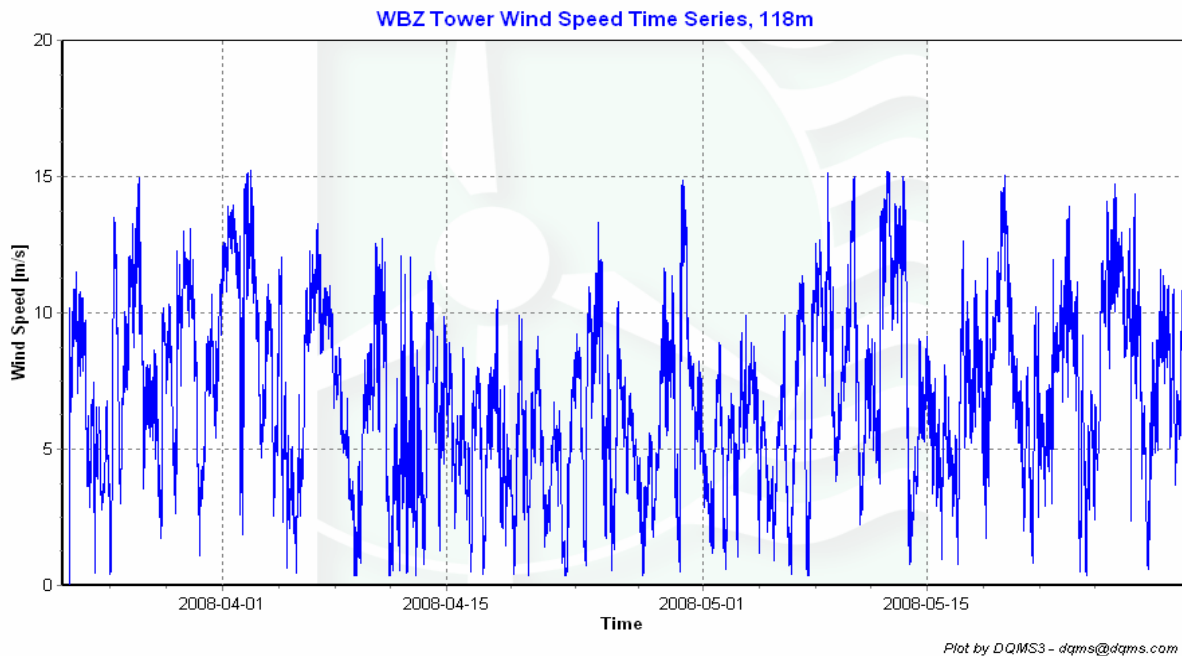
Figure 2 - WBZ Tower Wind Speed Time Series for March 22 to May 31
