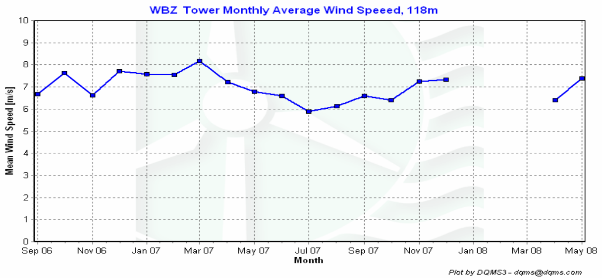
Figure 4 - WBZ Tower Monthly Average Wind Speed
