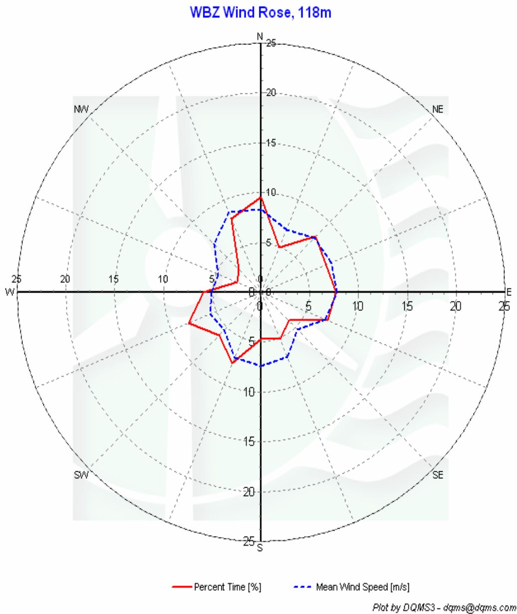
Figure 5 - WBZ Tower Wind Rose for March 22 to May 31
