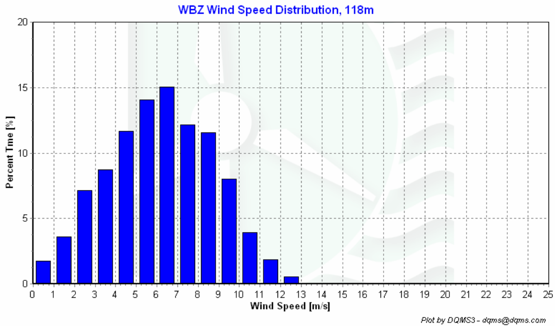
Figure 3 - WBZ Tower Wind Speed Distribution for June 1 to August 31
