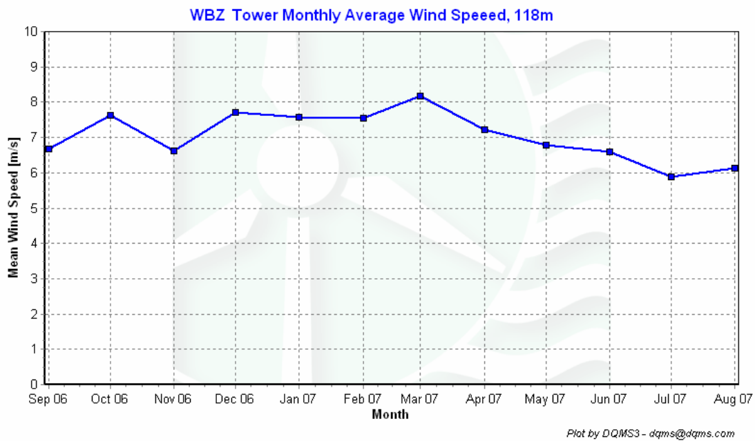
Figure 4 - WBZ Tower Monthly Average Wind Speed
