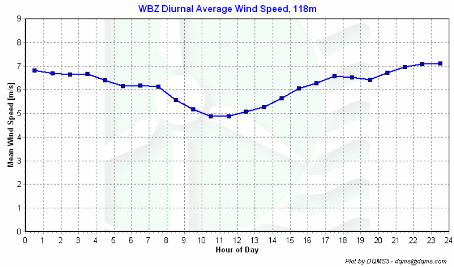
Figure 5 - WBZ Tower Diurnal Average Wind Speed for June 1 to August 31
