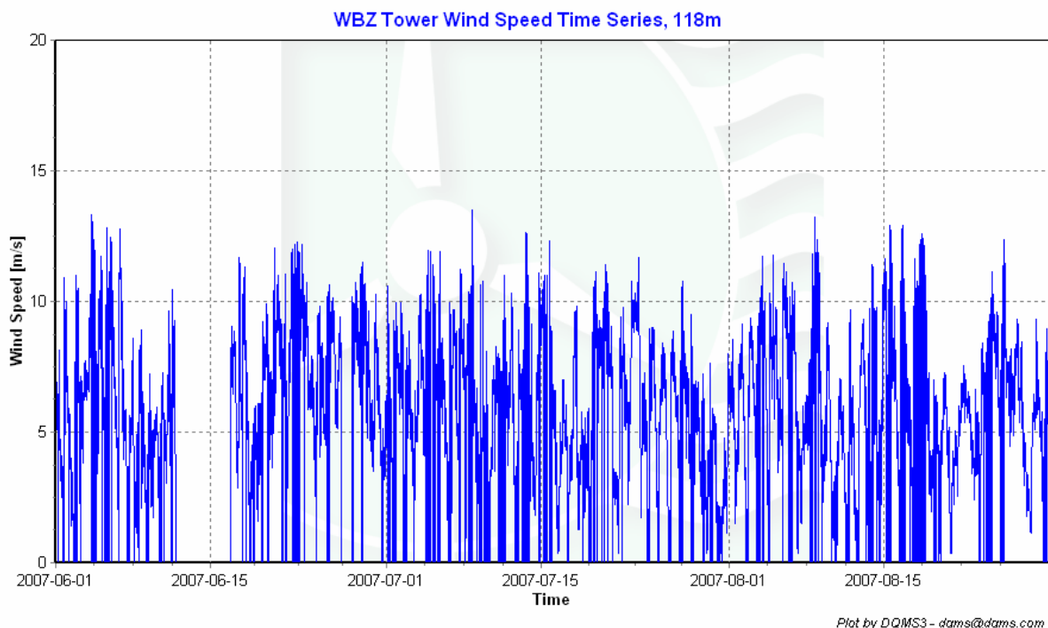
Figure 2 - WBZ Tower Wind Speed Time Series for June 1 to August 31
