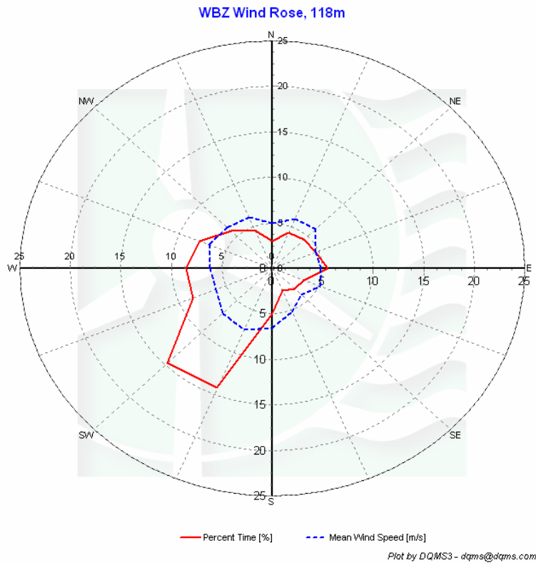
Figure 6 - WBZ Tower Wind Rose for June 1 to August 31
