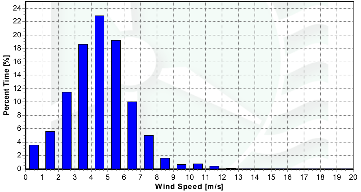
Figure 4: Wind speed distribution, July 2004 – September 2004
