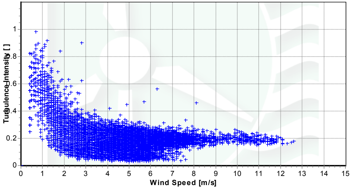
Figure 7: Turbulence Intensity vs. Wind Speed, July 2004 – September 2004
