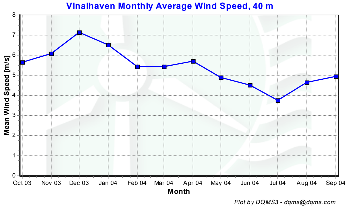
Figure 5: Average monthly wind speeds, October 2003 – September 2004
