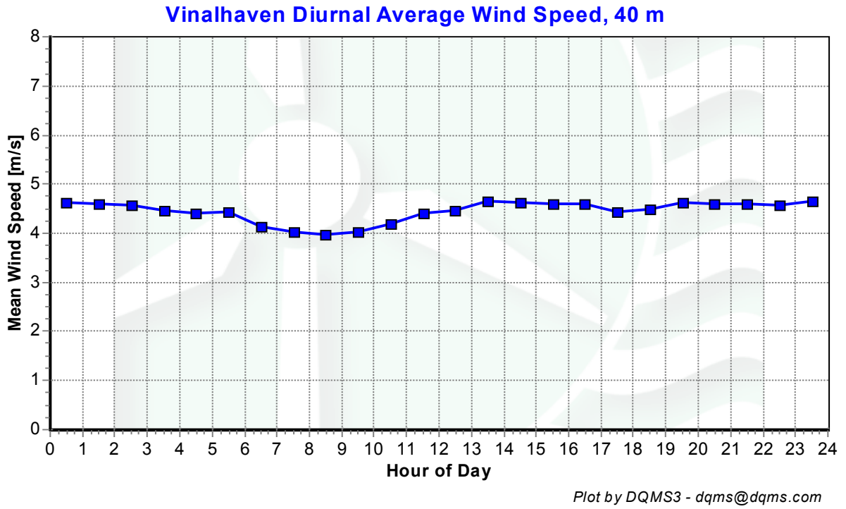
Figure 6: Diurnal average wind speeds, July 2004 – September 2004
