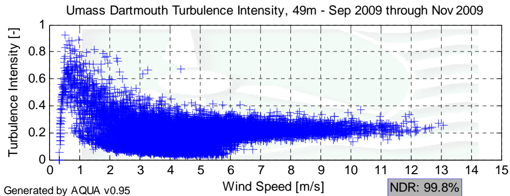
Figure 5 – Turbulence Intensity vs. Wind Speed, September 1, 2009 – November 30, 2009
