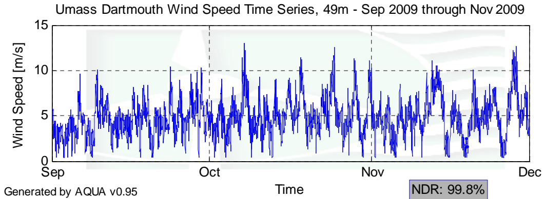
Figure 2 – Wind Speed Time Series, September 1, 2009 – November 30, 2009
