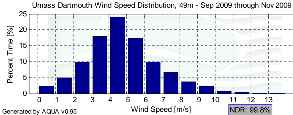
Figure 2 – Wind Speed Distribution, September 1, 2009 – November 30, 2009
