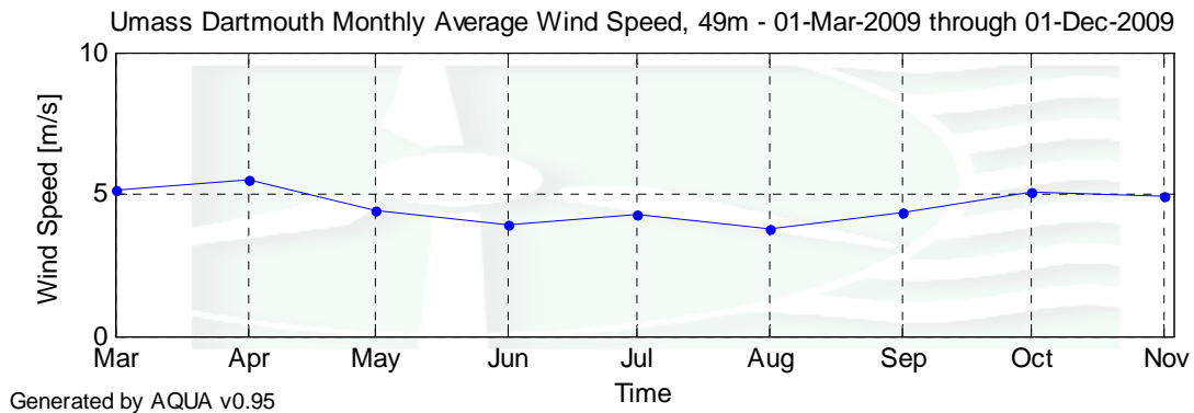
Figure 3 – Monthly Average Wind Speed, March 1, 2009 – November 30, 2009
