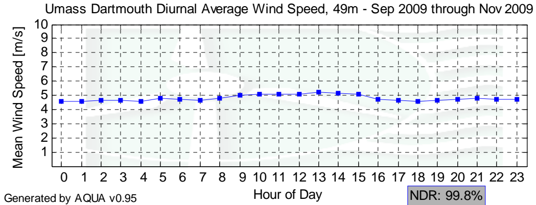
Figure 4 – Diurnal Average Wind Speeds, September 1, 2009 – November 30, 2009
