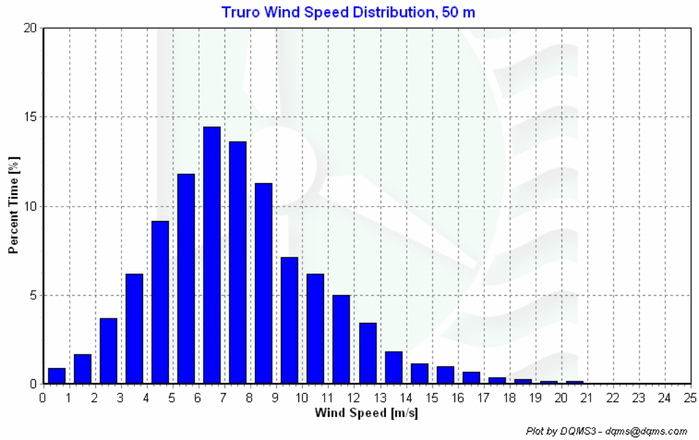
Figure 3 – Truro Wind Speed Distribution, September 1, 2006 - November 30, 2006
