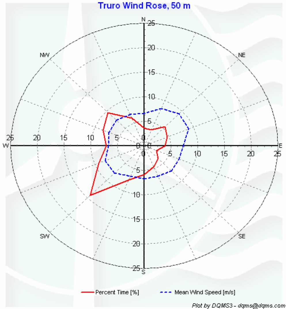
Figure 7 - Truro Wind Rose at 50 m, September 1, 2006 - November 30, 2006
