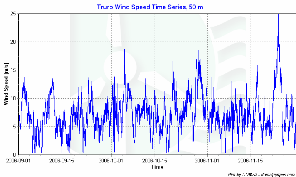
Figure 2 –Truro Wind Speed Time Series, September 1, 2006 - November 30, 2006
