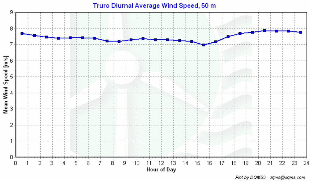
Figure 5 – Truro Diurnal Average Wind Speed at 50 m, September 1, 2006 - November 30, 2006
