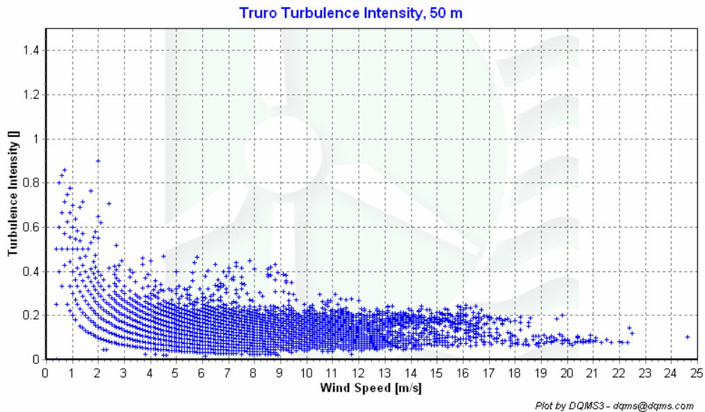
Figure 6 – Truro Turbulence Intensity at 50 m, September 1, 2006 - November 30, 2006
