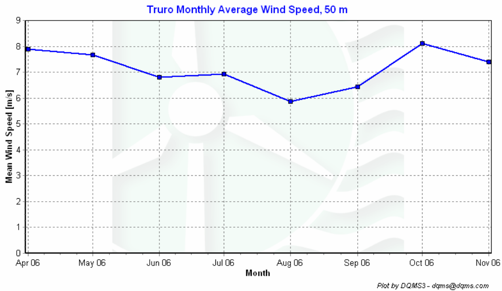
Figure 4 – Truro Monthly Average Wind Speed at 50 m, April 2006 - November 2006
