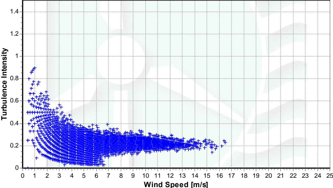
Figure 6 - Turbulence Intensity, March 1 st 2008 – May 31 st 2008
