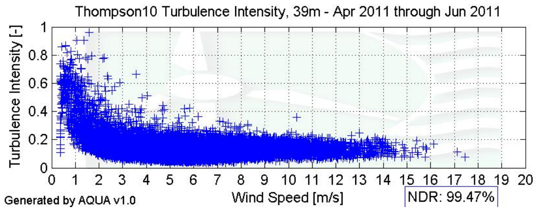
Figure 7 – Turbulence Intensity
