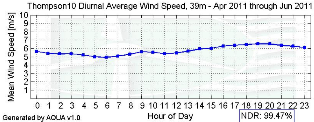
Figure 6 – Diurnal Average Wind Speeds
