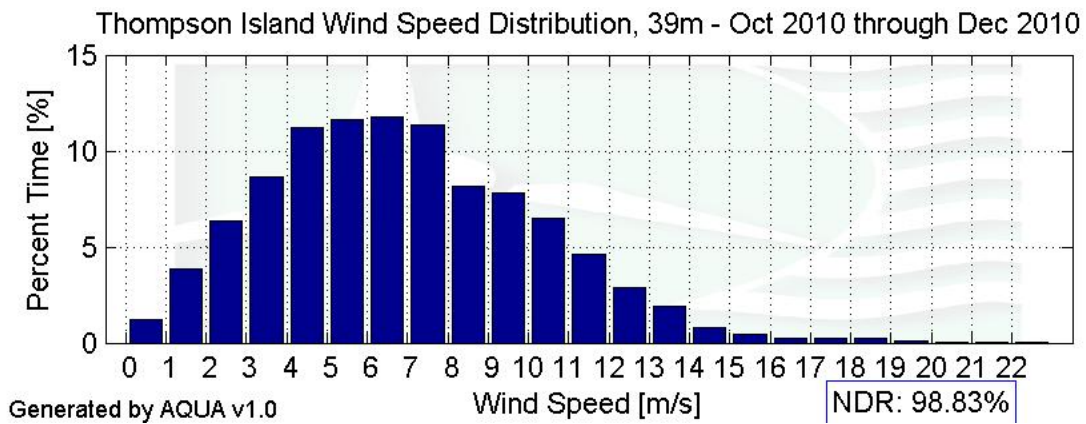
Figure 4 – Wind Speed Distribution, October 2010 - December 2010
