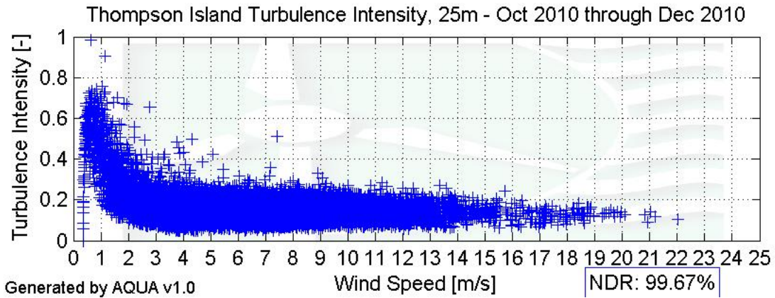
Figure 7 – Turbulence Intensity, October 2010 - December 2010
