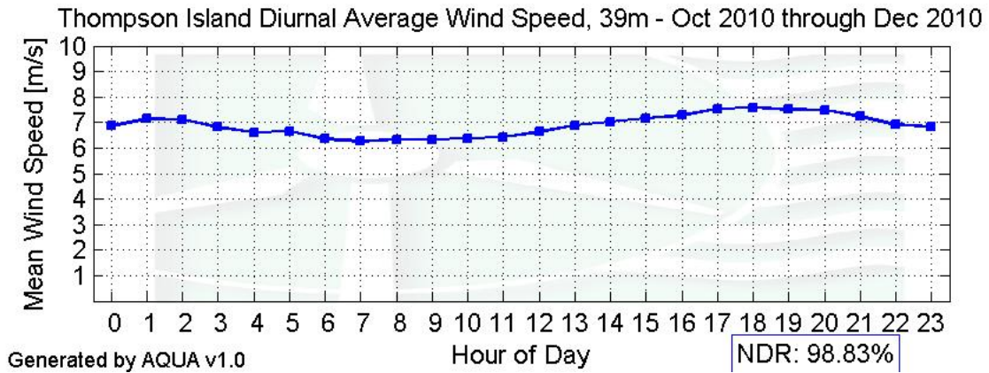
Figure 6 – Diurnal Average Wind Speeds, October 2010 - December 2010
