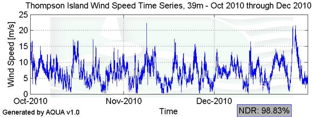
Figure 3 – Wind Speed Time Series, October 2010 - December 2010
