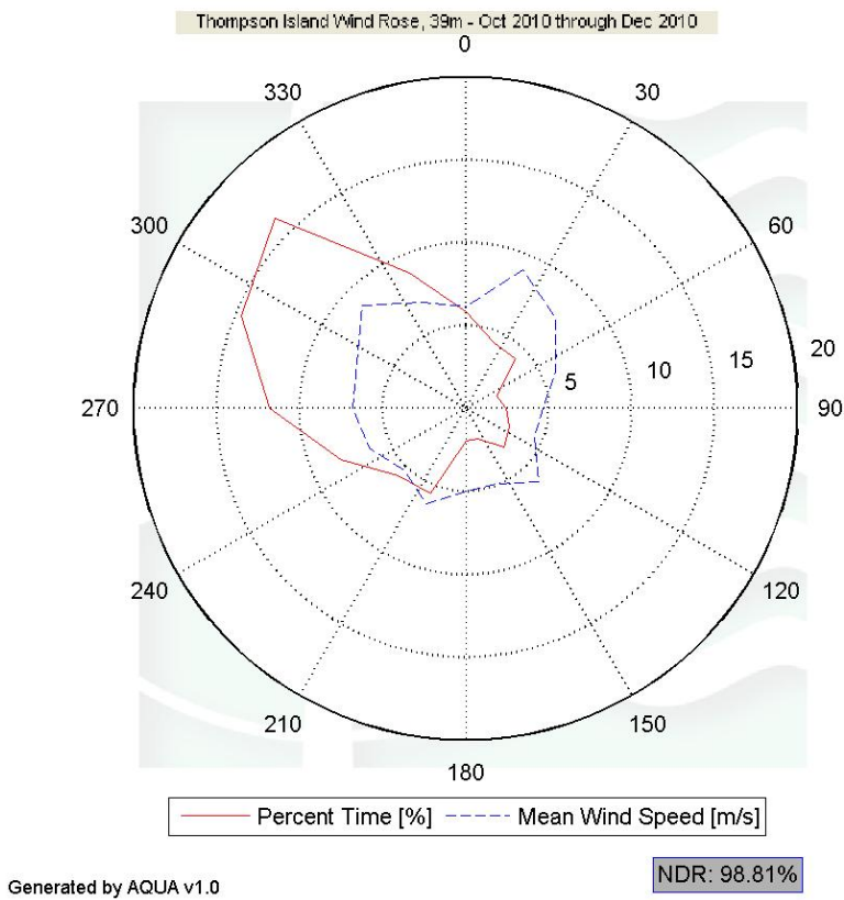
Figure 8 – Wind Rose, October 2010 - December 2010
