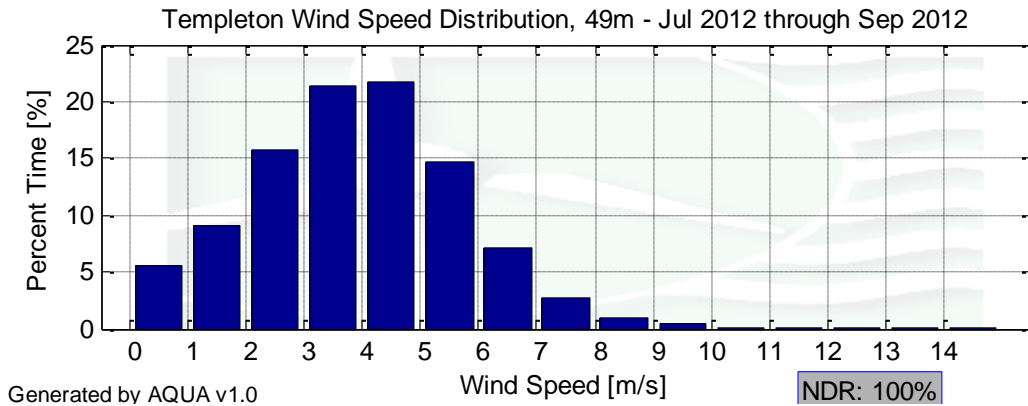
Figure 3 – Templeton Wind Speed Distribution for July 1 to September 30, 2012
