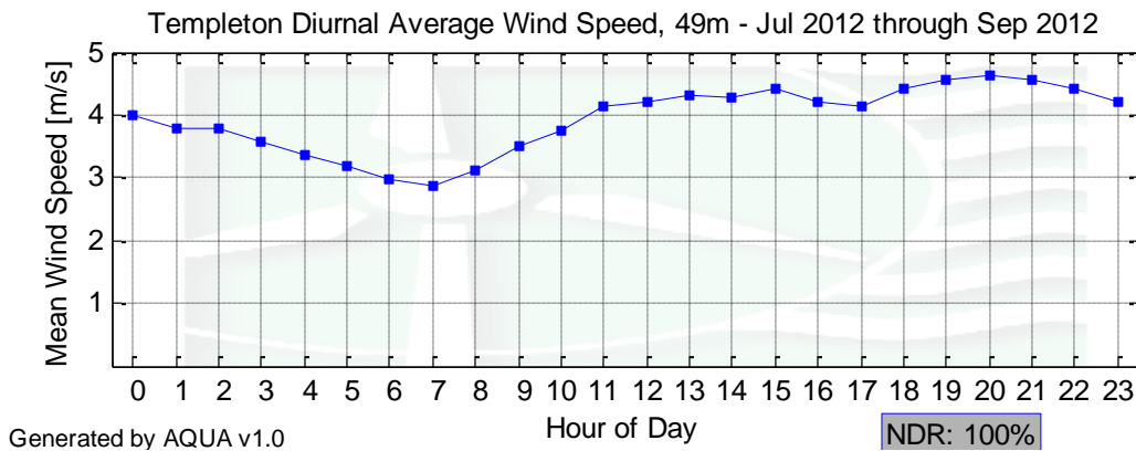
Figure 5 – Templeton Diurnal Average Wind Speeds for July 1 to September 30, 2012
