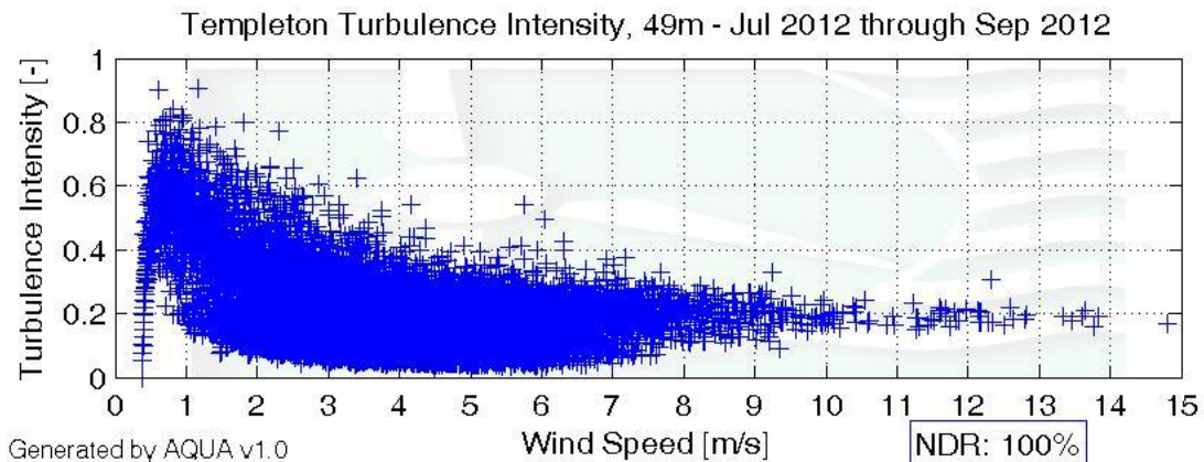
Figure 6 – Templeton Turbulence Intensity for July 1 to September 30, 2012
