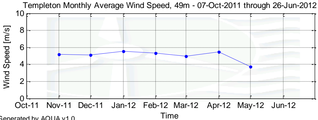
Figure 4 – Templeton Monthly Wind Speed Averages for October 7, 2011 to June 30, 2012
