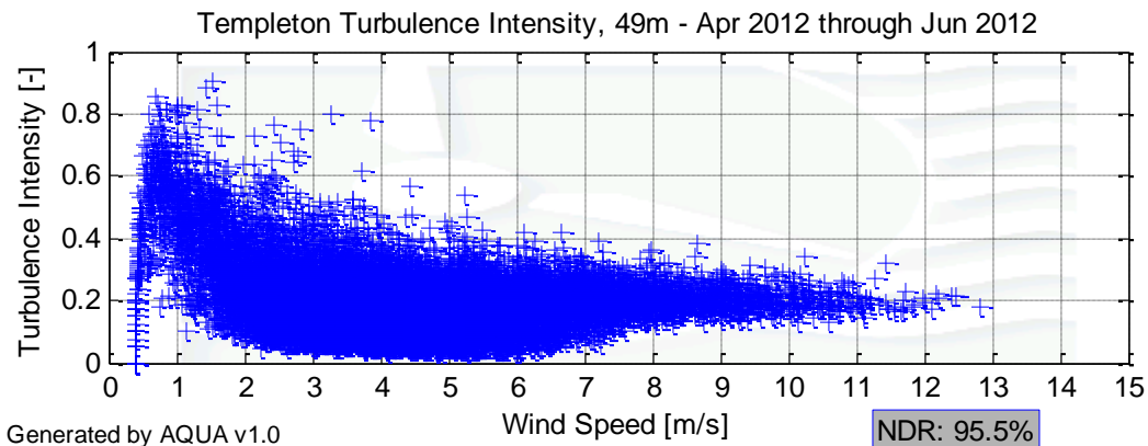
Figure 6 – Templeton Turbulence Intensity for April 1 to June 30, 2012
