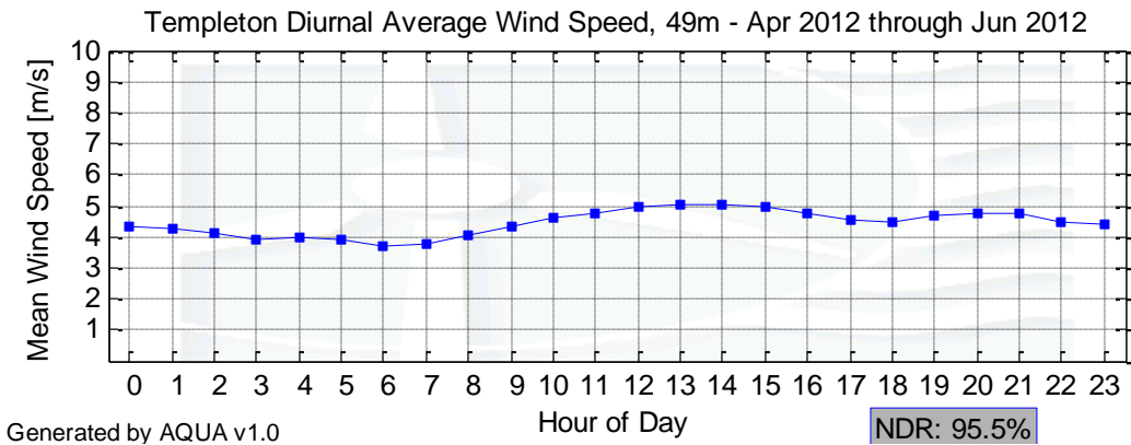
Figure 5 – Templeton Diurnal Average Wind Speeds for April 1 to June 30, 2012
