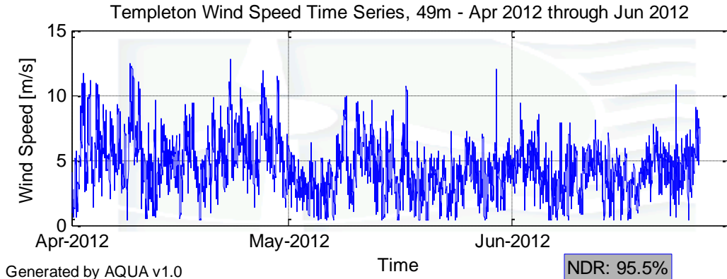
Figure 2 – Templeton Wind Speed Time Series for April 1 to June 30, 2012
