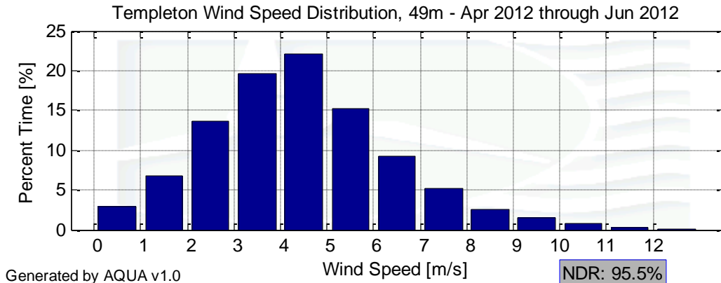
Figure 3 – Templeton Wind Speed Distribution for April 1 to June 30, 2012
