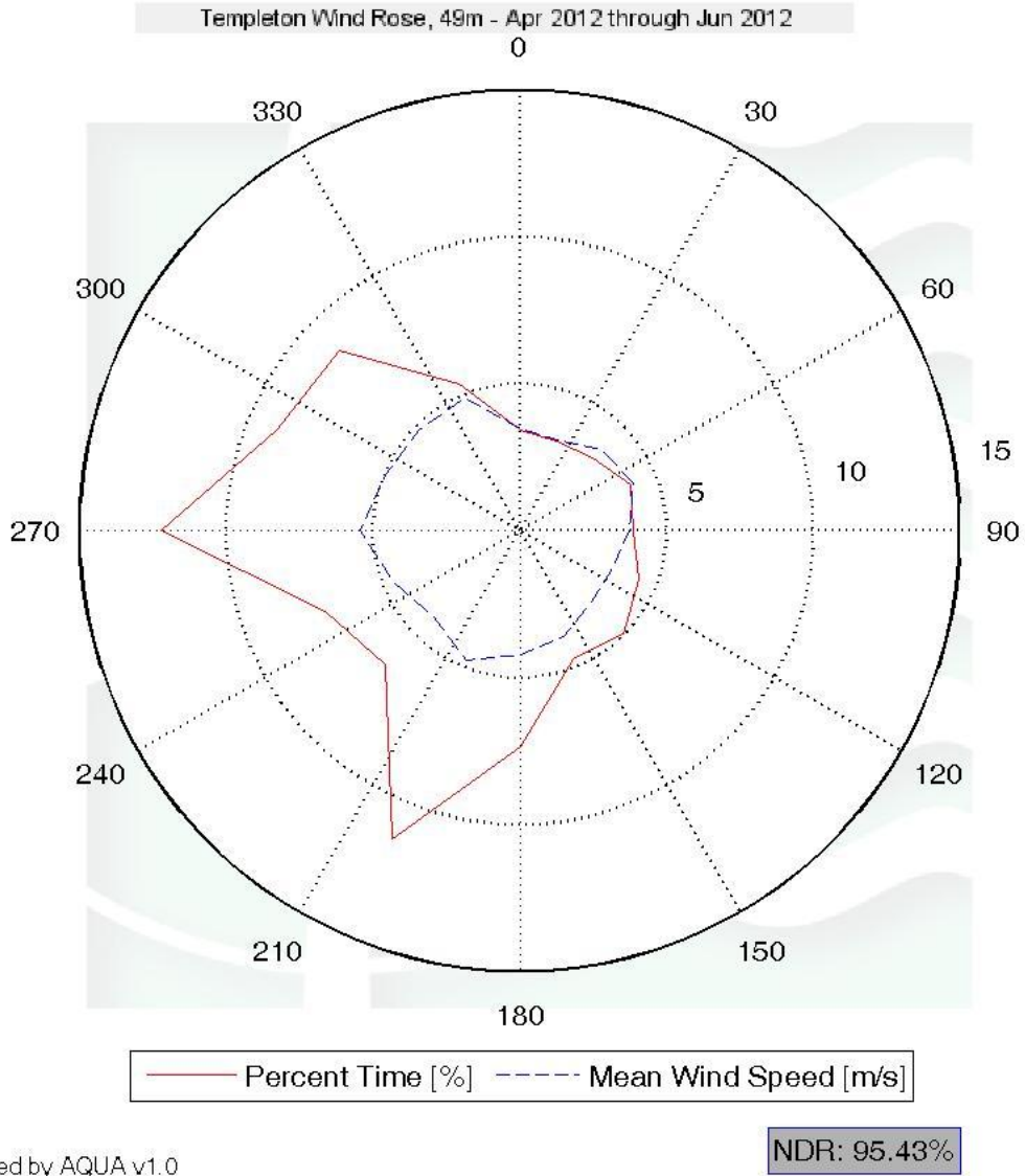
Figure 7 – Templeton Wind Rose for April 1 to June 30, 2012
