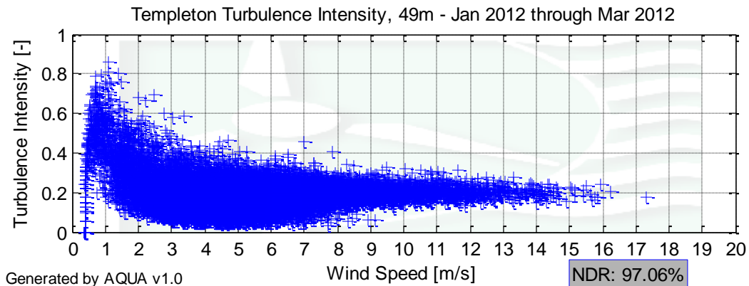
Figure 6 – Templeton Turbulence Intensity for January 1 to March 31, 2012
