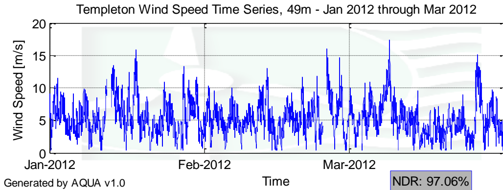
Figure 2 – Templeton Wind Speed Time Series for January 1 to March 31, 2012
