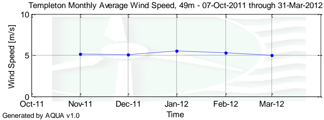
Figure 4 – Templeton Monthly Wind Speed Averages for October 7, 2011 to March 31, 2012
