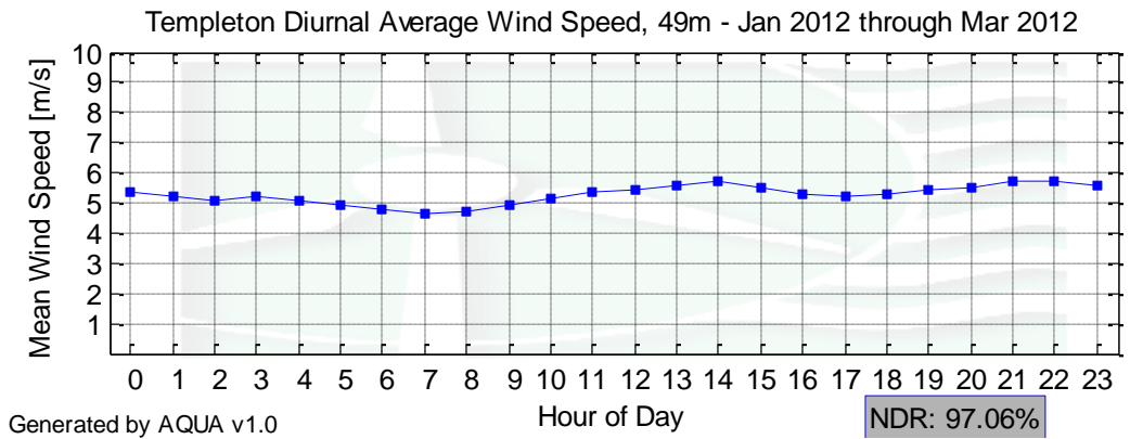
Figure 5 – Templeton Diurnal Average Wind Speeds for January 1 to March 31, 2012
