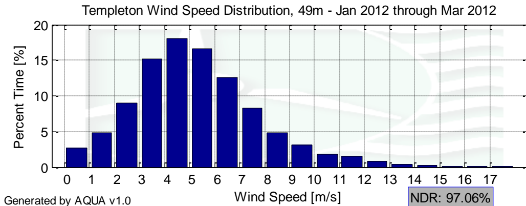
Figure 3 – Templeton Wind Speed Distribution for January 1 to March 31, 2012
