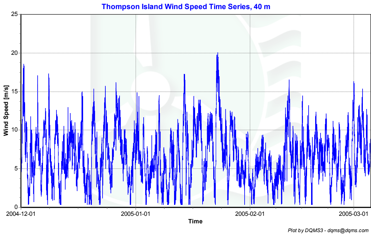
Figure 3 - Wind Speed Time Series, December 2004 – February 2005
