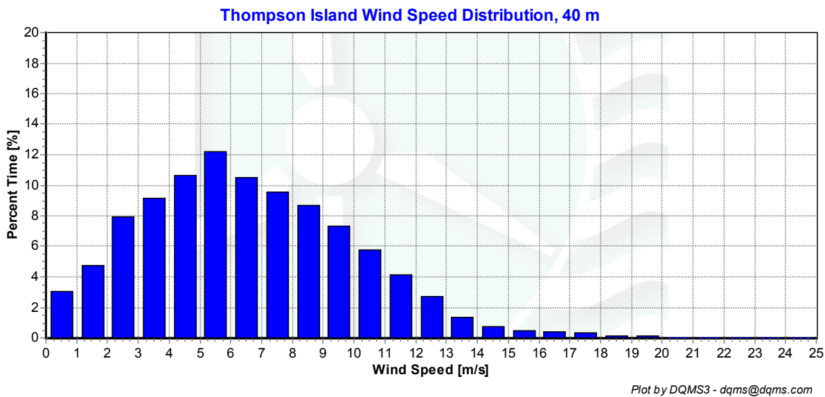
Figure 4 - Wind Speed Distribution, December 2004 – February 2005
