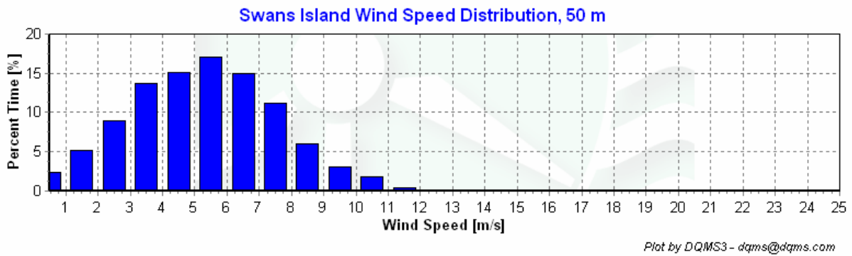
Figure 3 – Wind Speed Distribution, June 1, 2008 – August 31, 2008
