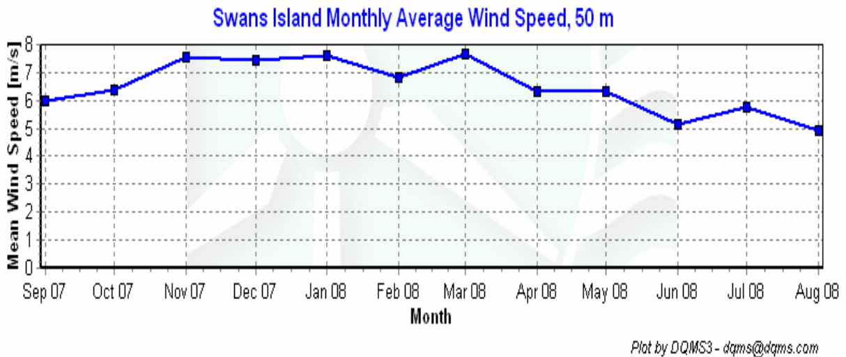
Figure 4 – Monthly Average Wind Speed September 2007 – August 2008
