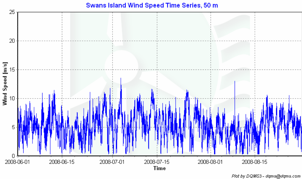
Figure 2 – Wind Speed Time Series, June 1, 2008 – August 31, 2008
