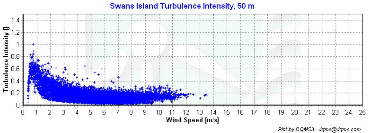
Figure 6 – Turbulence Intensity, June 1, 2008 – August 31, 2008
