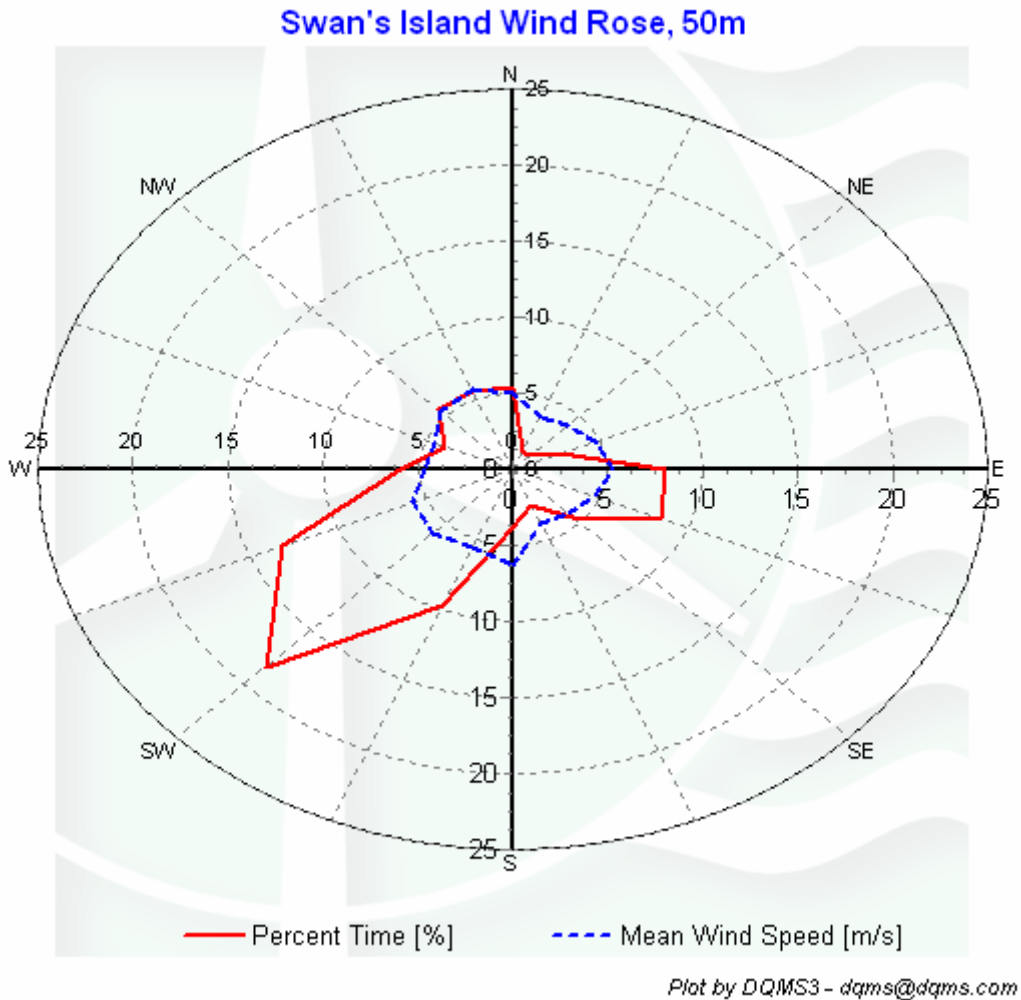
Figure 7 – Wind Rose, June 1, 2008 – August 31, 2008
