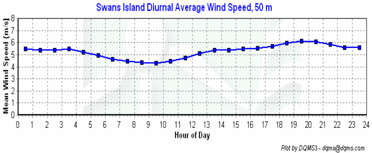
Figure 5 – Diurnal Average Wind Speed, June 1, 2008 – August 31, 2008
