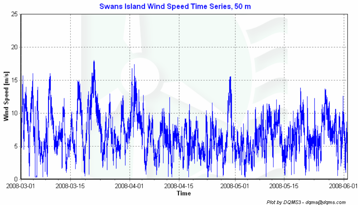
Figure 2 – Wind Speed Time Series, March 1, 2008 – May 31, 2008
