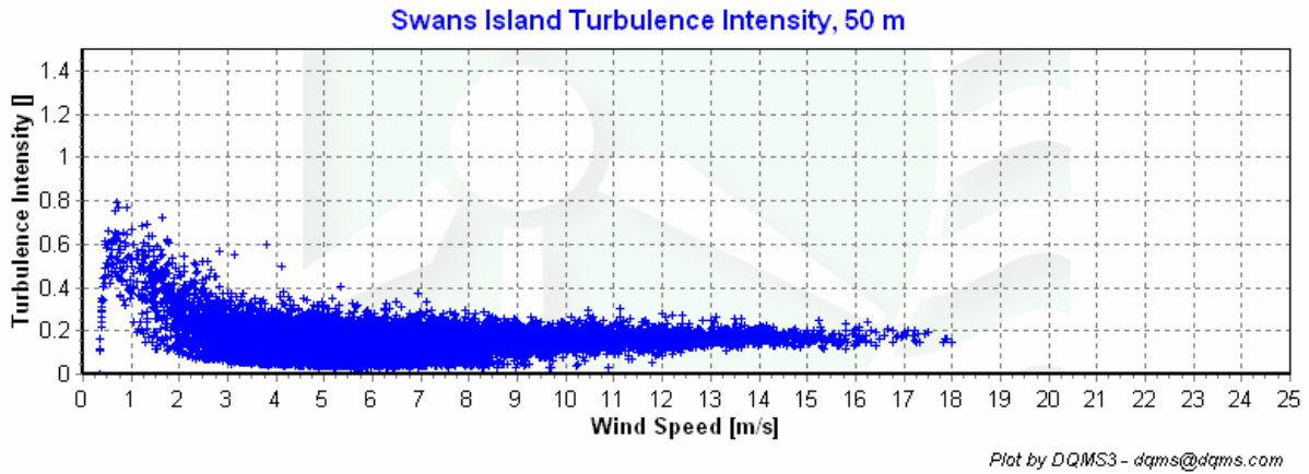
Figure 6 – Turbulence Intensity, March 1, 2008 – May 31, 2008
