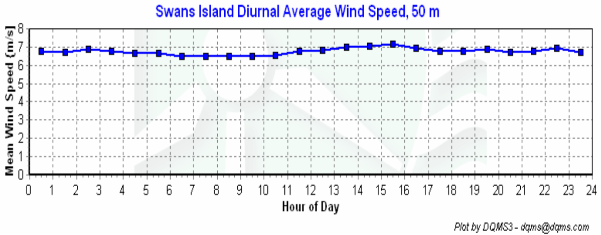
Figure 5 – Diurnal Average Wind Speed, March 1, 2008 – May 31, 2008
