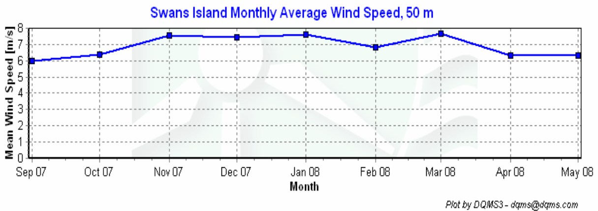
Figure 4 – Monthly Average Wind Speed September 2007 – May 2008
