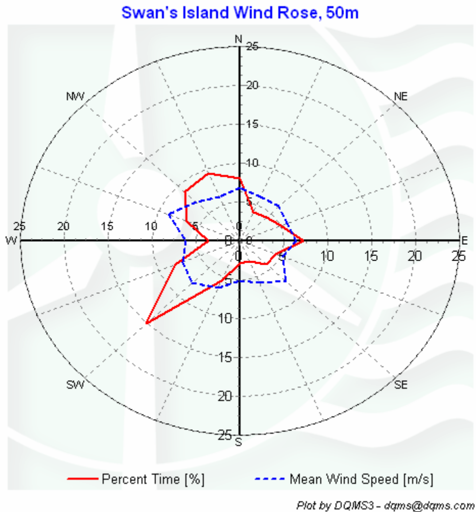
Figure 7 – Wind Rose, March 1, 2008 – May 31, 2008
