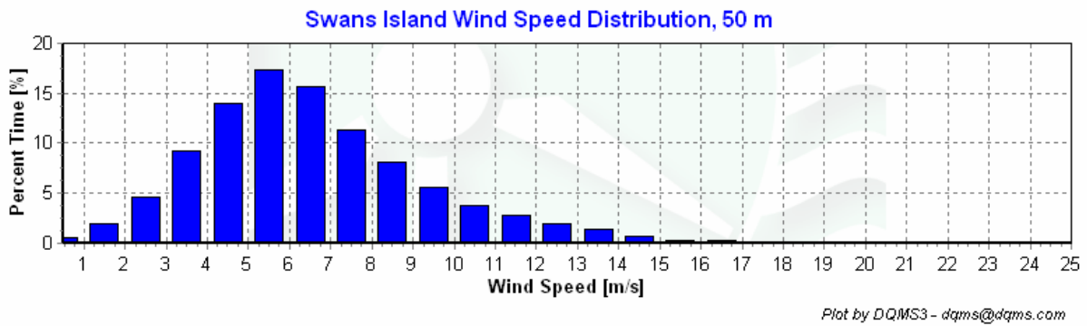
Figure 3 – Wind Speed Distribution, September 1, 2008 – November 30, 2008
