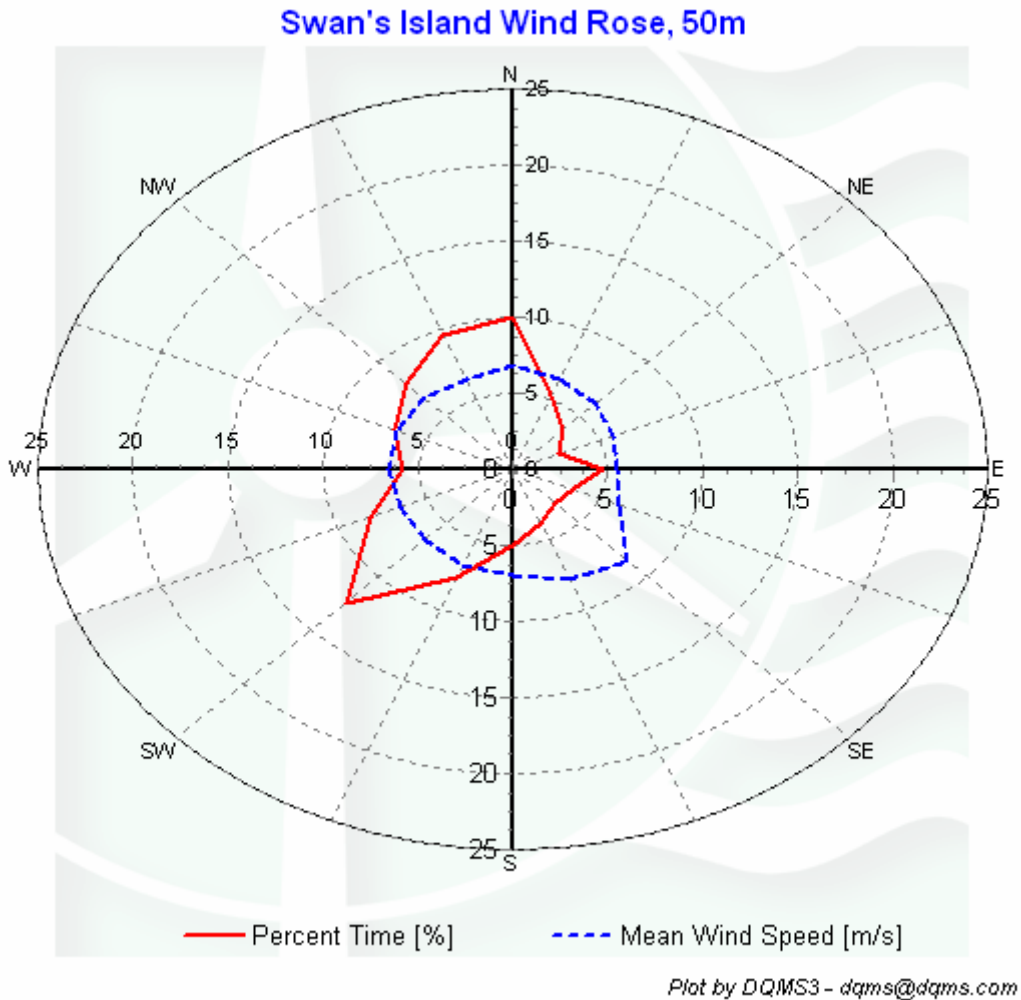
Figure 7 – Wind Rose, September 1, 2008 – November 30, 2008
