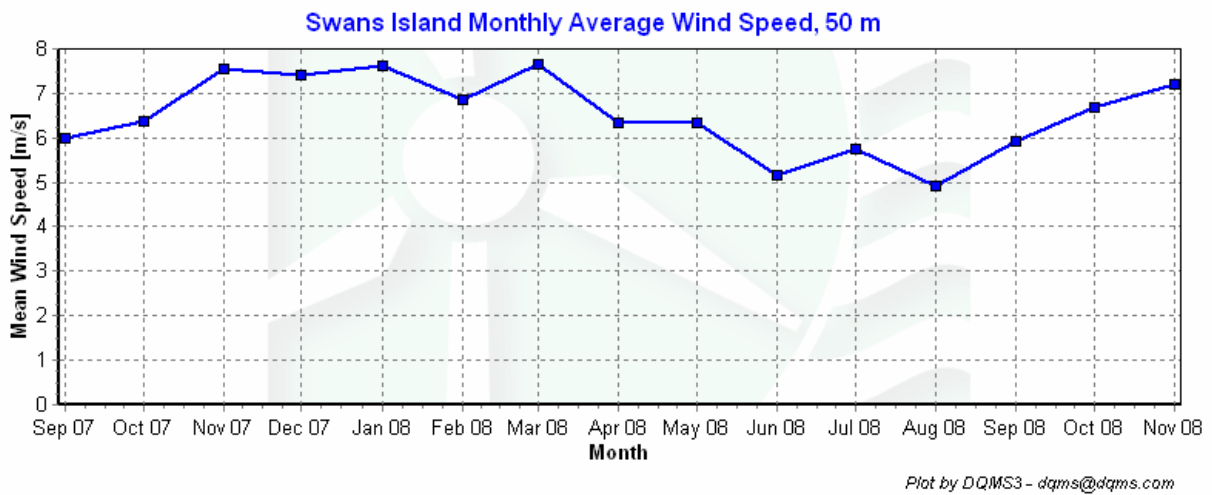
Figure 4 – Monthly Average Wind Speed September 2007 – November 2008
