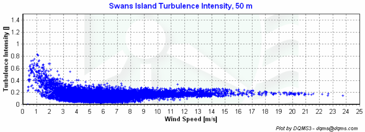
Figure 6 – Turbulence Intensity, September 1, 2008 – November 30, 2008
