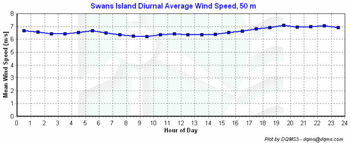
Figure 5 – Diurnal Average Wind Speed, September 1, 2008 – November 30, 2008
