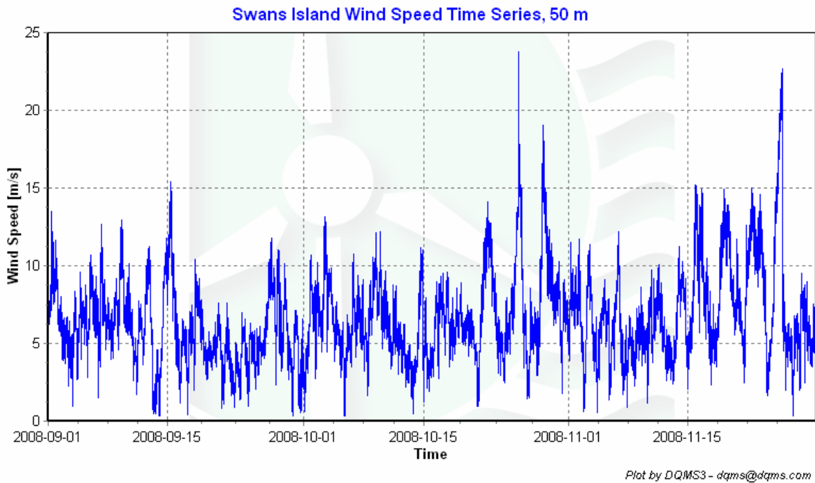
Figure 2 – Wind Speed Time Series, September 1, 2008 – November 30, 2008
