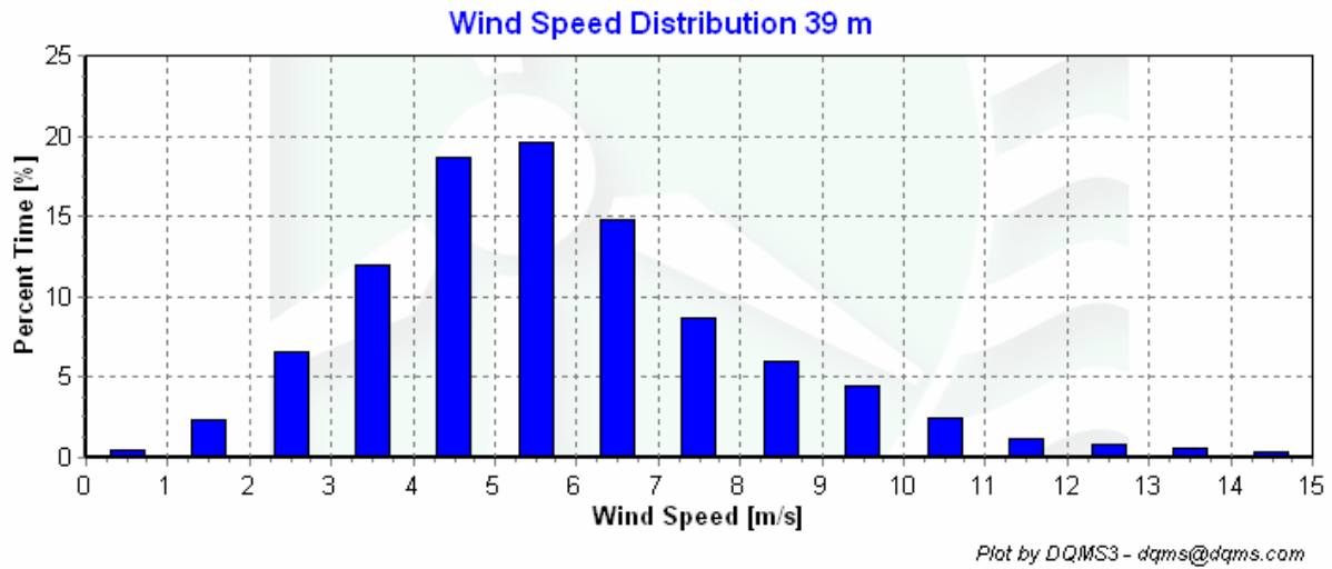
Figure 3 – Wind Speed Distribution, September 1, 2006 – November 30, 2006
