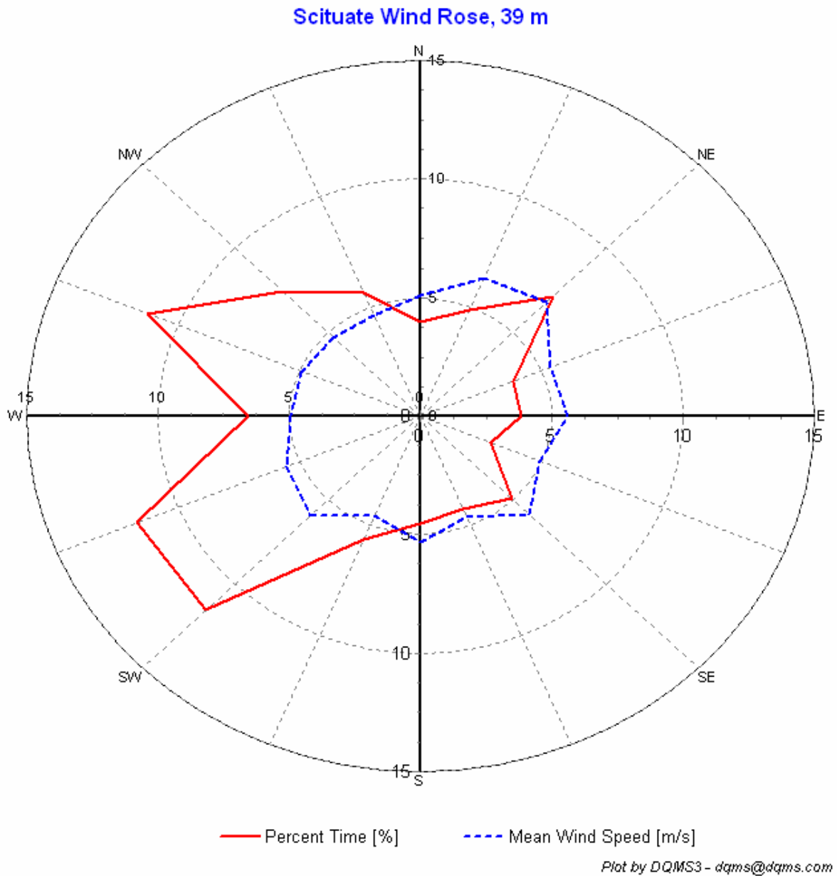
Figure 7 – Wind Rose, September 1, 2006 – November 30, 2006
