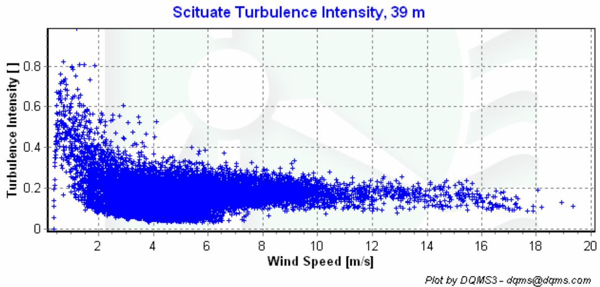
Figure 6 – Turbulence Intensity vs. Wind Speed, September 1, 2006 – November 30, 2006
