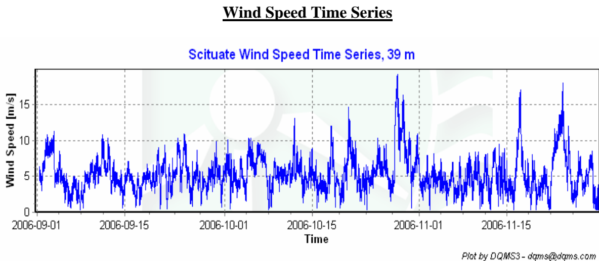
Figure 2 – Wind Speed Time Series, September 1, 2006 – November 30, 2006
