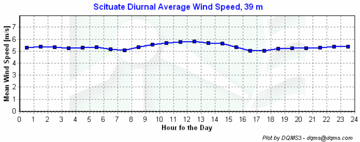
Figure 5 – Diurnal Wind Speed, September 1, 2006 – November 30, 2006
