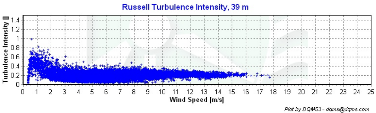
Figure 6 – Turbulence Intensity vs. Wind Speed, December 1, 2009 – February 28, 2010
