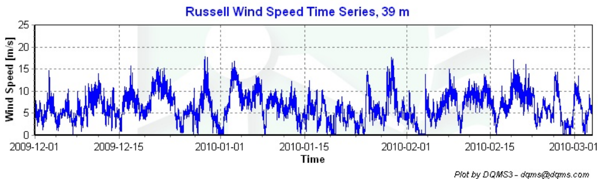
Figure 2 – Wind Speed Time Series, December 1, 2009 – February 28, 2010
