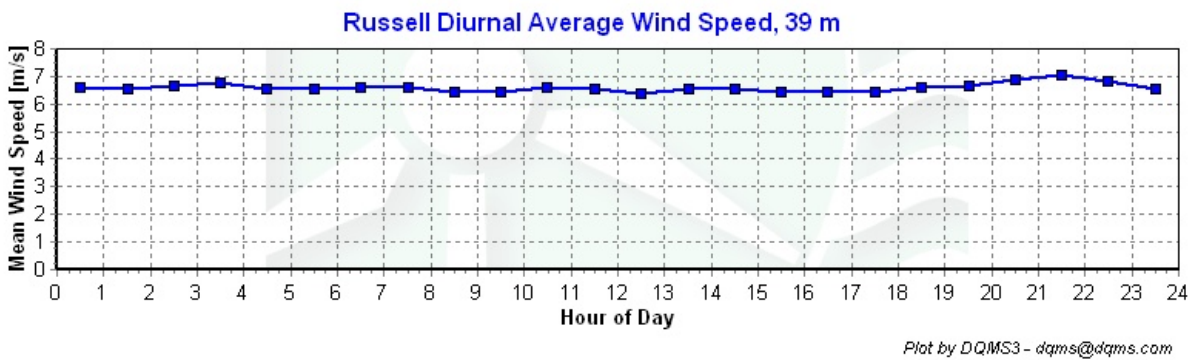
Figure 5 – Diurnal Average Wind Speeds, December 1, 2009 – February 28, 2010
