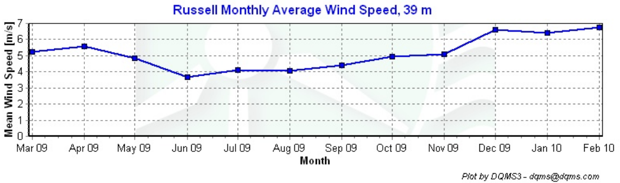
Figure 4 – Monthly Average Wind Speed, March, 2009 – February 2010
