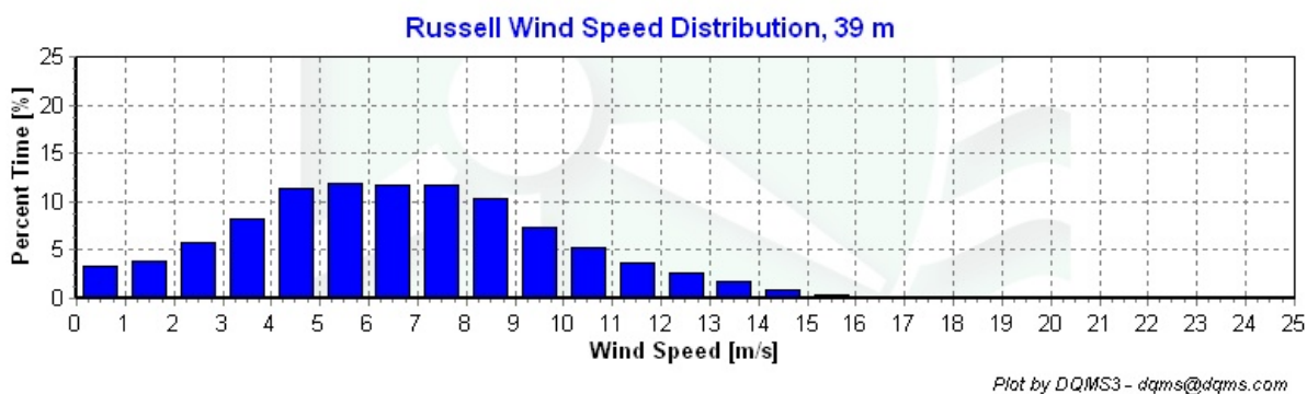
Figure 3 – Wind Speed Distribution, December 1, 2009 – February 28, 2010
