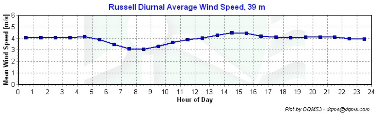
Figure 5 – Diurnal Average Wind Speeds, June 1, 2009 – August 31, 2009
