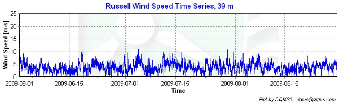
Figure 2 – Wind Speed Time Series, June 1, 2009 – August 31, 2009
