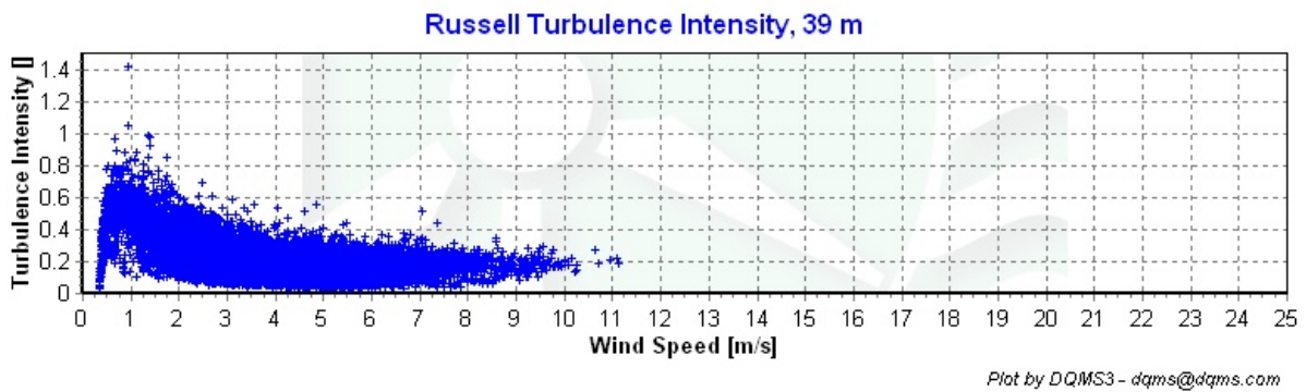
Figure 6 – Turbulence Intensity vs. Wind Speed, June 1, 2009 – August 31, 2009
