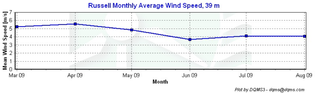
Figure 4 – Monthly Average Wind Speed, March, 2009 – August, 2009
