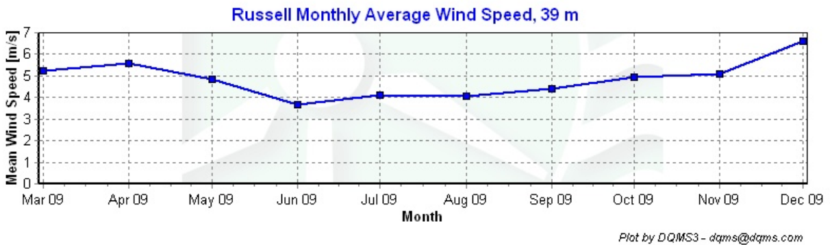
Figure 4 – Monthly Average Wind Speed, March, 2009 – December, 2009
