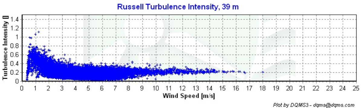
Figure 6 – Turbulence Intensity vs. Wind Speed, September 1, 2009 – November 30, 2009
