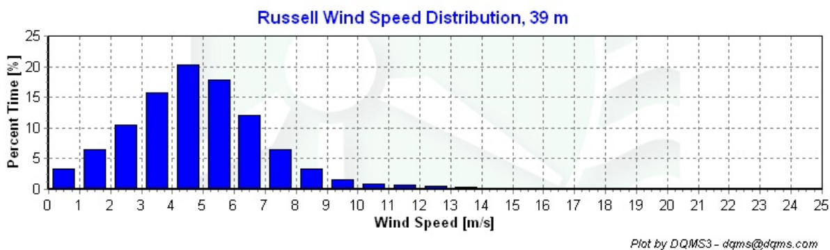
Figure 3 – Wind Speed Distribution, September 1, 2009 – November 30, 2009
