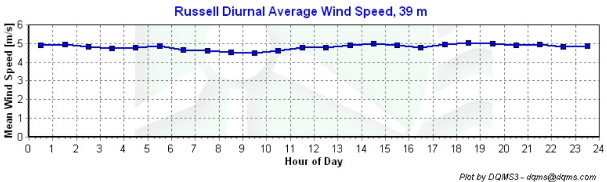
Figure 5 – Diurnal Average Wind Speeds, September 1, 2009 – November 30, 2009
