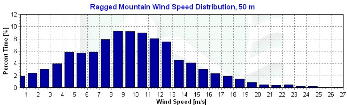
Figure 3– Wind Speed Distribution, Dec 1, 2007 – February 9, 2008.
