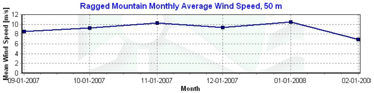
Figure 4– Monthly Average Wind Speeds, Dec 1, 2007 – February 9, 2008.
