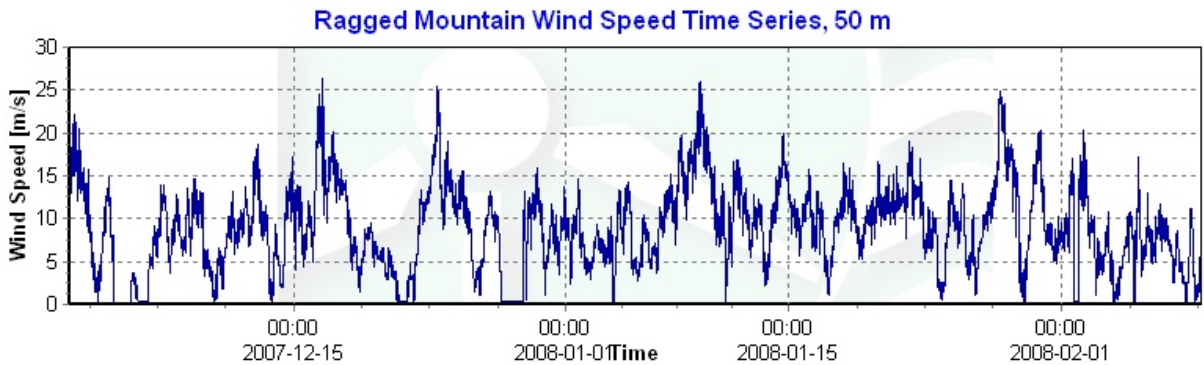
Figure 2– Wind Speed Time Series, Dec 1, 2007 – February 9, 2008.
