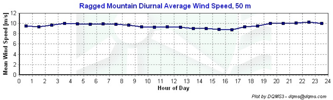
Figure 5– Diurnal Average Wind Speeds, Dec 1, 2007 – February 9, 2008.
