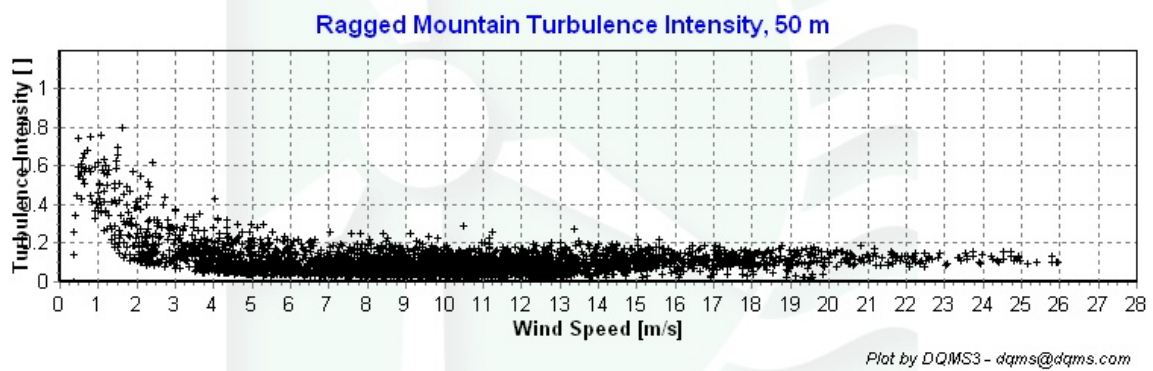
Figure 6– Turbulence Intensity vs. Wind Speed, Dec 1, 2007 – February 9, 2008.
