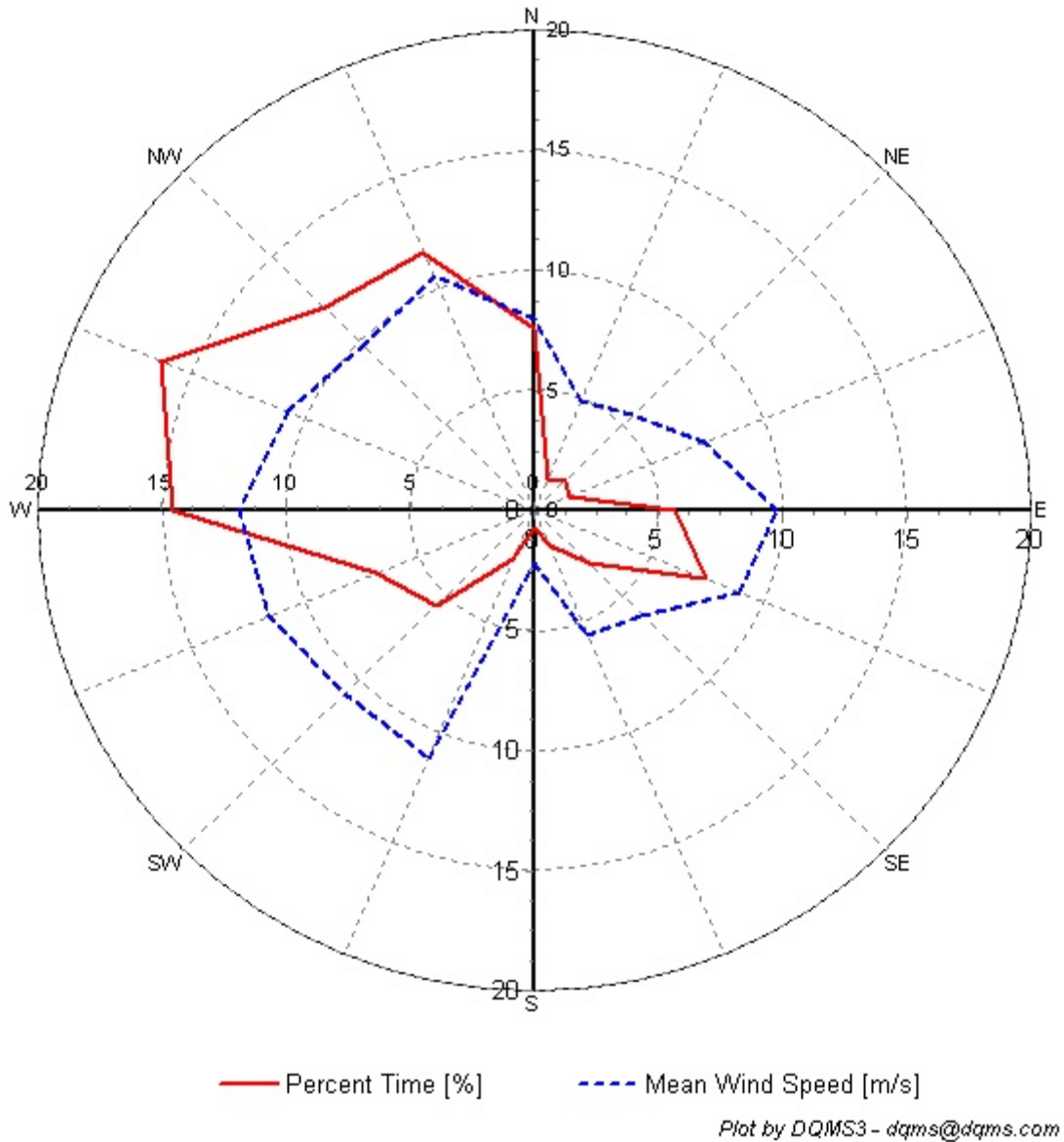
Figure 7– Wind Rose, Dec 1, 2007 – February 9, 2008.
