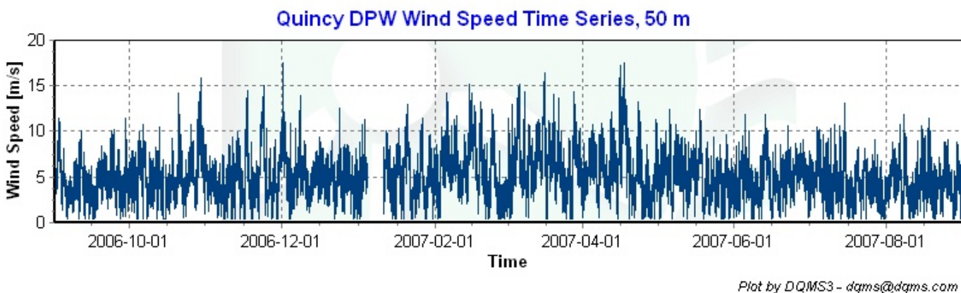
Figure 2– Wind Speed Time Series, September 1, 2006 – August 31, 2007.
