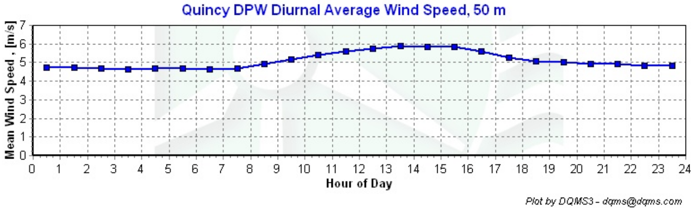
Figure 5– Diurnal Average Wind Speeds, September 1, 2006 – August 31, 2007.
