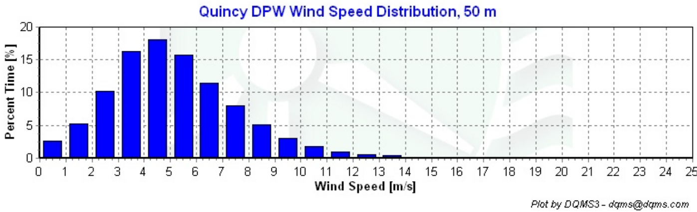
Figure 3– Wind Speed Distribution, September 1, 2006 – August 31, 2007.
