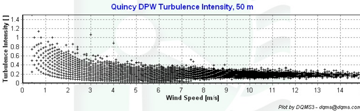
Figure 6– Turbulence Intensity vs. Wind Speed, September 1, 2006 – August 31, 2007.
