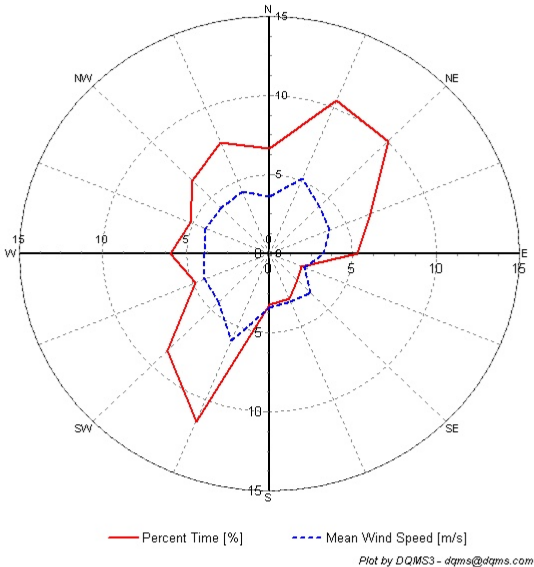
Figure 6 – Wind Rose, August 10, 2006 – August 31, 2006.
