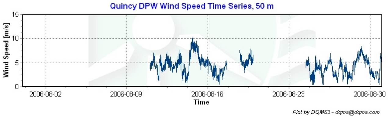
Figure 2 – Wind Speed Time Series, August 1, 2006 – August 31, 2006.
