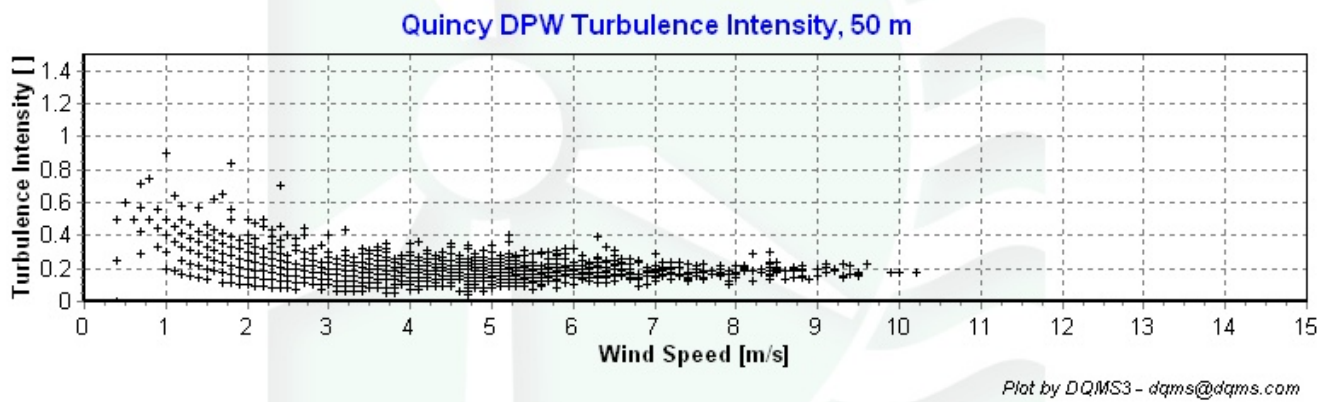
Figure 5 – Turbulence Intensity vs. Wind Speed, August 10, 2006 – August 31, 2006.
