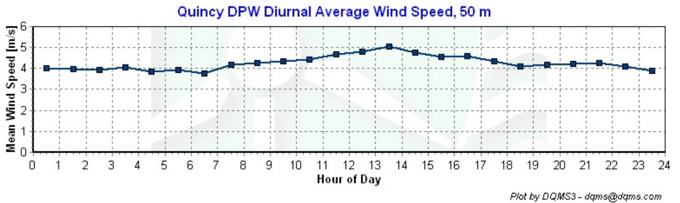
Figure 4 – Diurnal Average Wind Speeds, August 10, 2006 – August 31, 2006.
