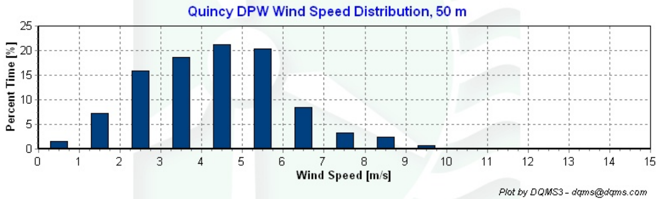
Figure 3 – Wind Speed Distribuion, Aug 10, 2006 – August 31, 2006.
