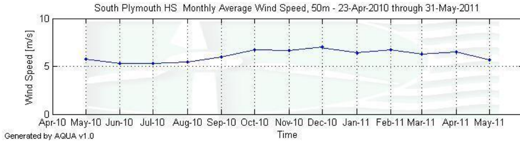
Figure 4 – Monthly Average Wind Speed, May 2010 - May 2011
