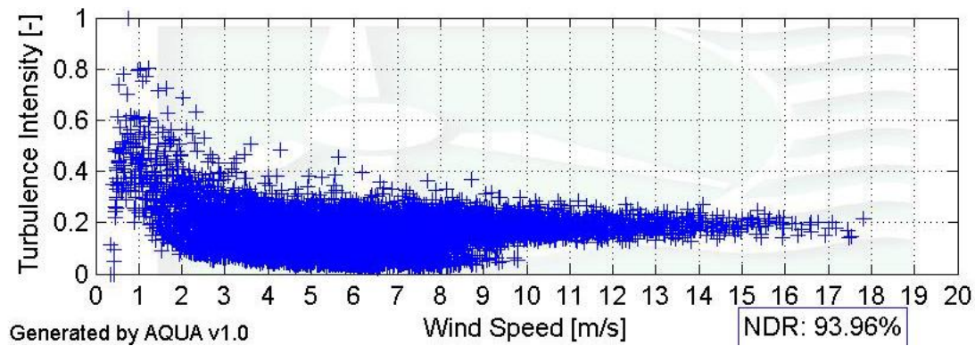
Figure 6 – Turbulence Intensity, May 2010 - May 2011
