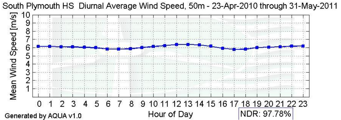
Figure 5 – Diurnal Average Wind Speed, May 2011 - May 2011
