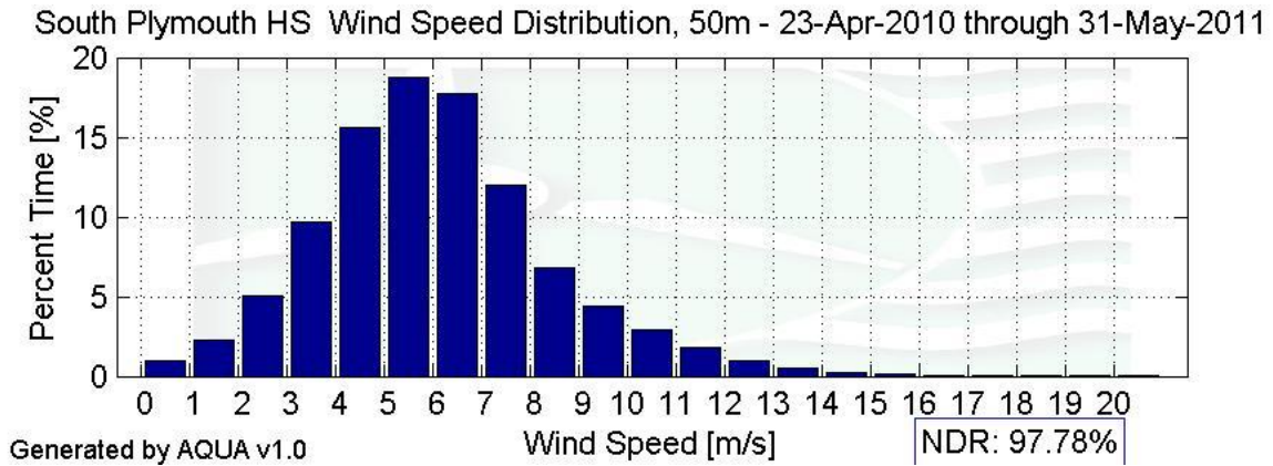
Figure 3 – Wind Speed Distribution, May 2010 - May 2011
