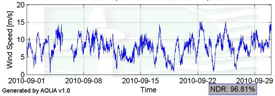
Paxton Wind Speed Time Series, 78m - Sep 2010
