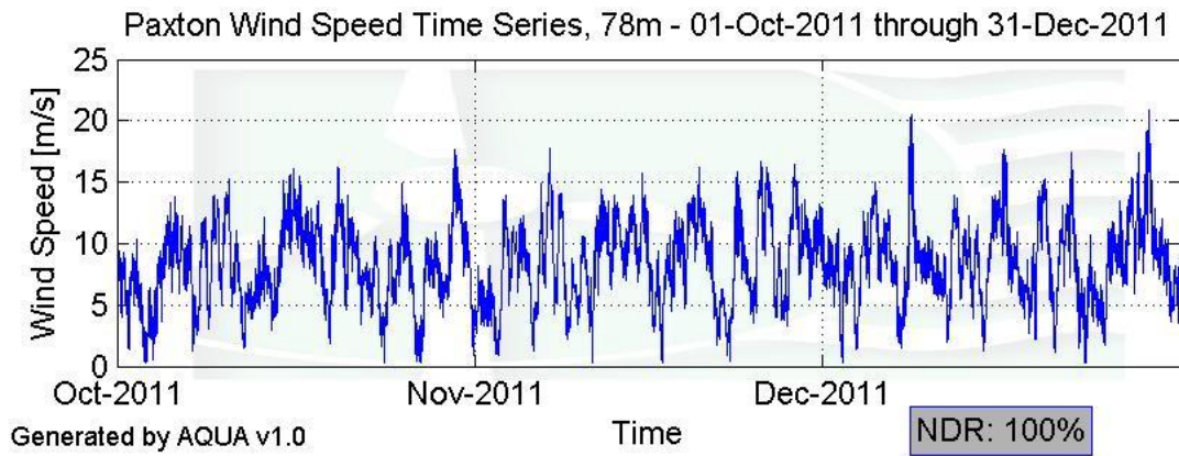
Figure 4- Wind Speed Time Series, October 2011 - December 2011
