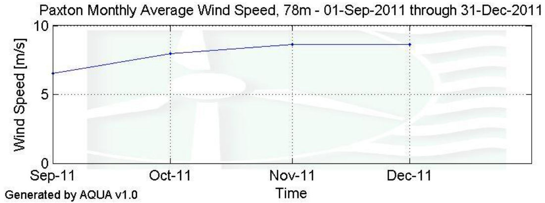
Figure 6 - Monthly Average Wind Speed, October 2011 - December 2011
