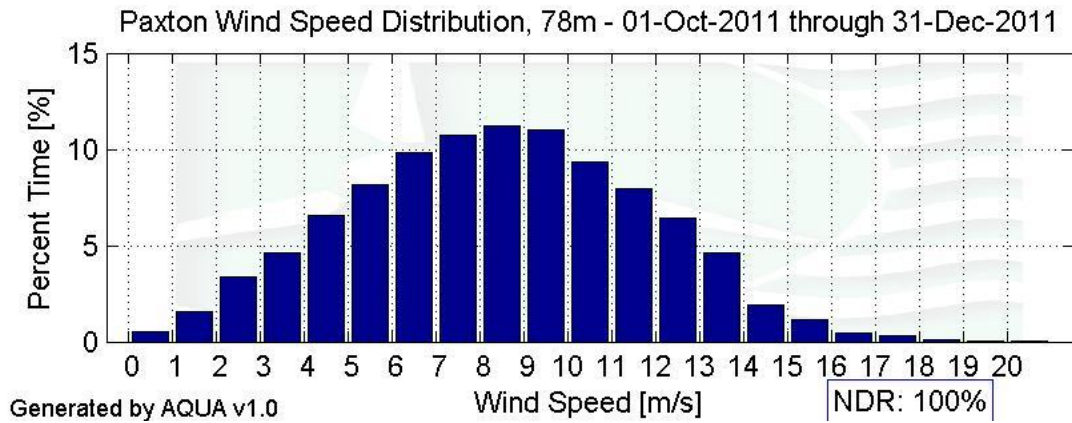
Figure 5- Wind Speed Distribution, October 2011 - December 2011
