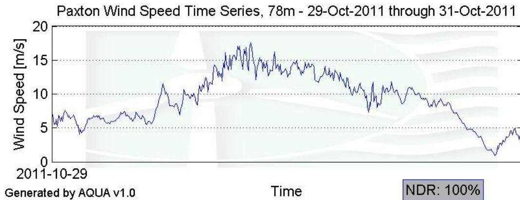
Figure 10 – Time series wind data for the weekend on October 29-30 during the October Snowstorm.
