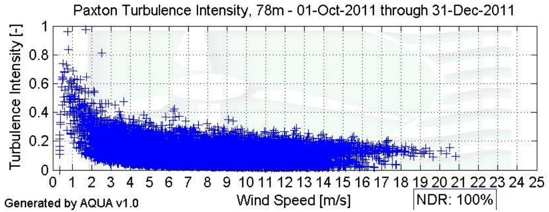
Figure 8 - Turbulence Intensity, October 2011 - December 2011
