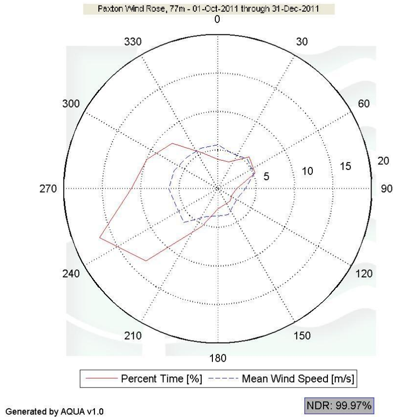
Figure 9 – Wind Rose October 2011 - December 2011
