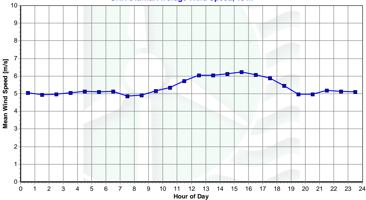
ORR Diurnal Average Wind Speed, 49 m
