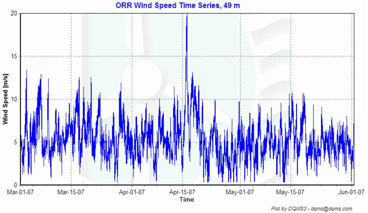
Figure 3 - Wind Speed Time Series, March 1 st 2007—May 31 st 2007
