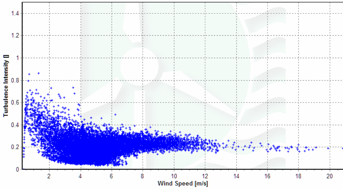
Figure 7 - Turbulence Intensity, March 1 st 2007—May 31 st 2007
