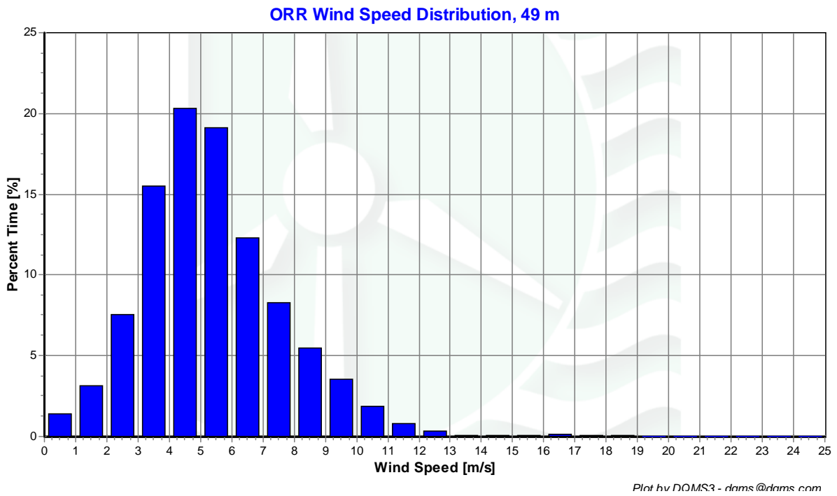
Figure 4 - Wind Speed Distribution, March 1 st 2007—May 31 st 2007
