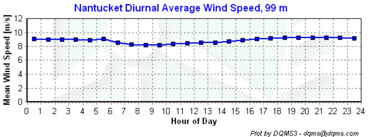
Figure 5 - Diurnal Wind Speed, June 1, 2006 - August 31, 2006.
