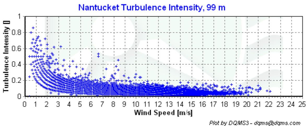
Figure 6 - Turbulence Intensity vs. Wind Speed, June 1, 2006 - August 31, 2006.
