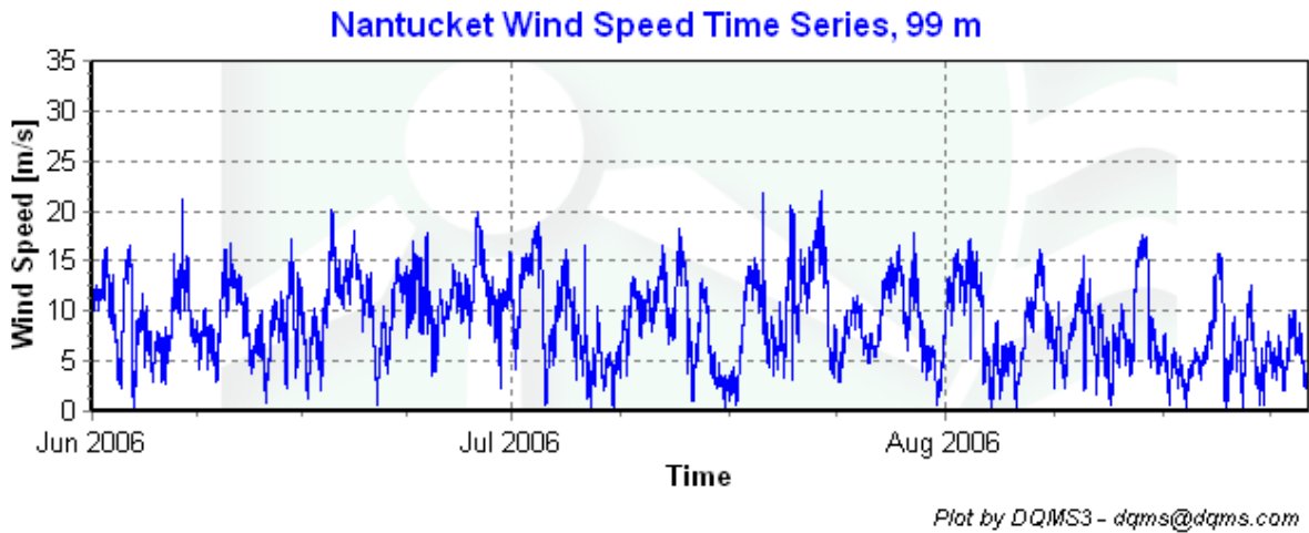
Figure 2 - Wind Speed Time Series, June 1, 2006 - August 31, 2006.
