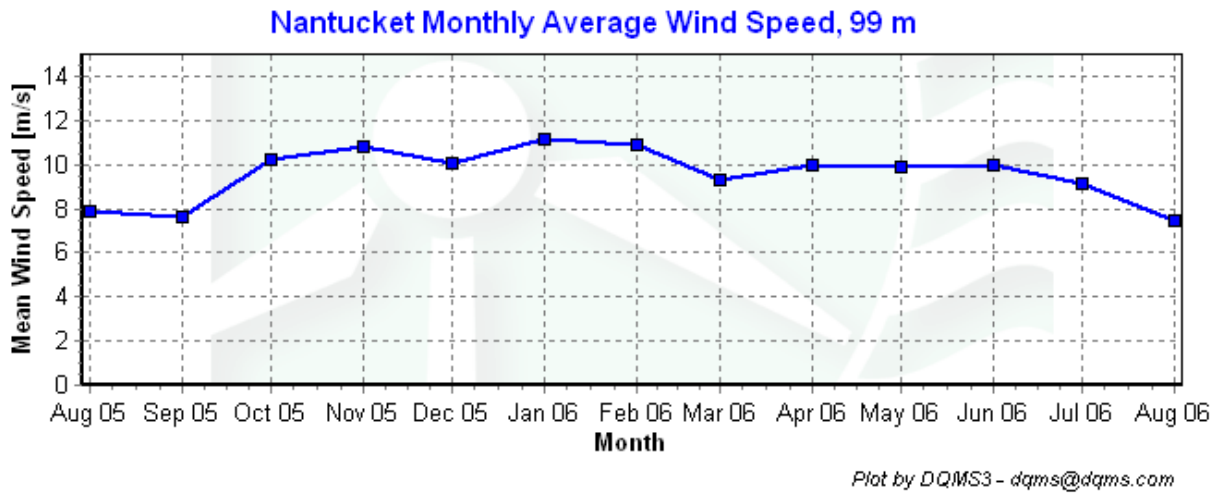
Figure 4 - Monthly Average Wind Speeds, August, 2005 - August, 2006.
