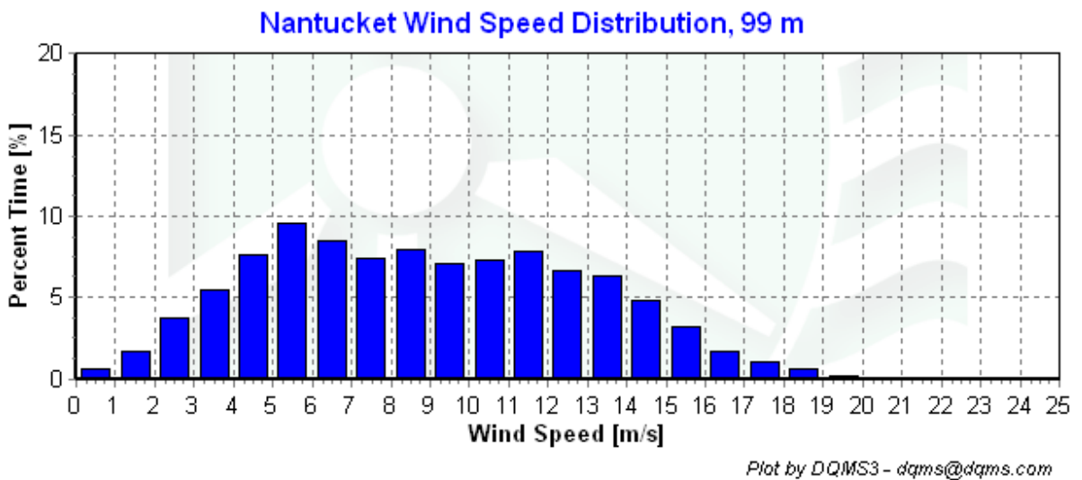
Figure 3 - Wind Speed Distribution, June 1, 2006 - August 31, 2006.
