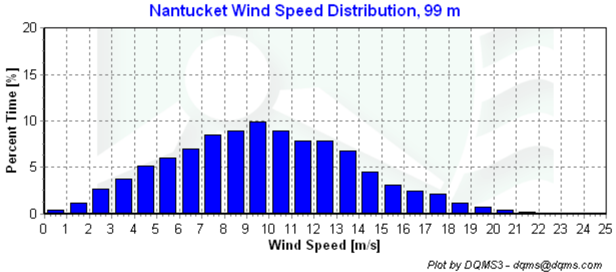
Figure 3 - Wind Speed Distribution, March 1, 2006 - May 31, 2006.
