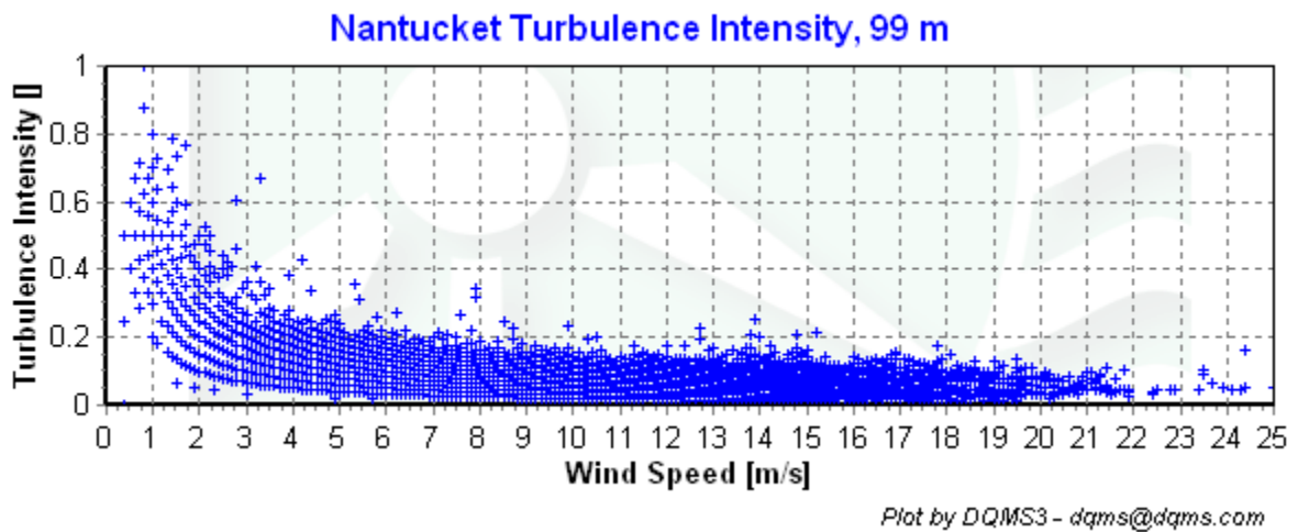
Figure 6 - Turbulence Intensity vs. Wind Speed, March 1, 2006 - May 31, 2006.
