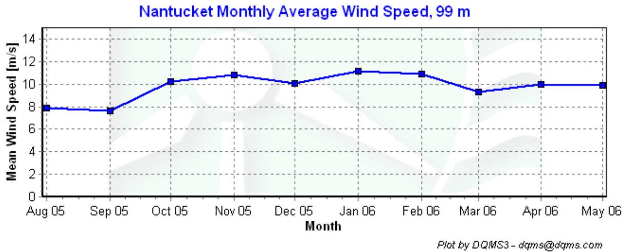
Figure 4 - Monthly average wind speeds, August 1, 2005 - May 31, 2006.
