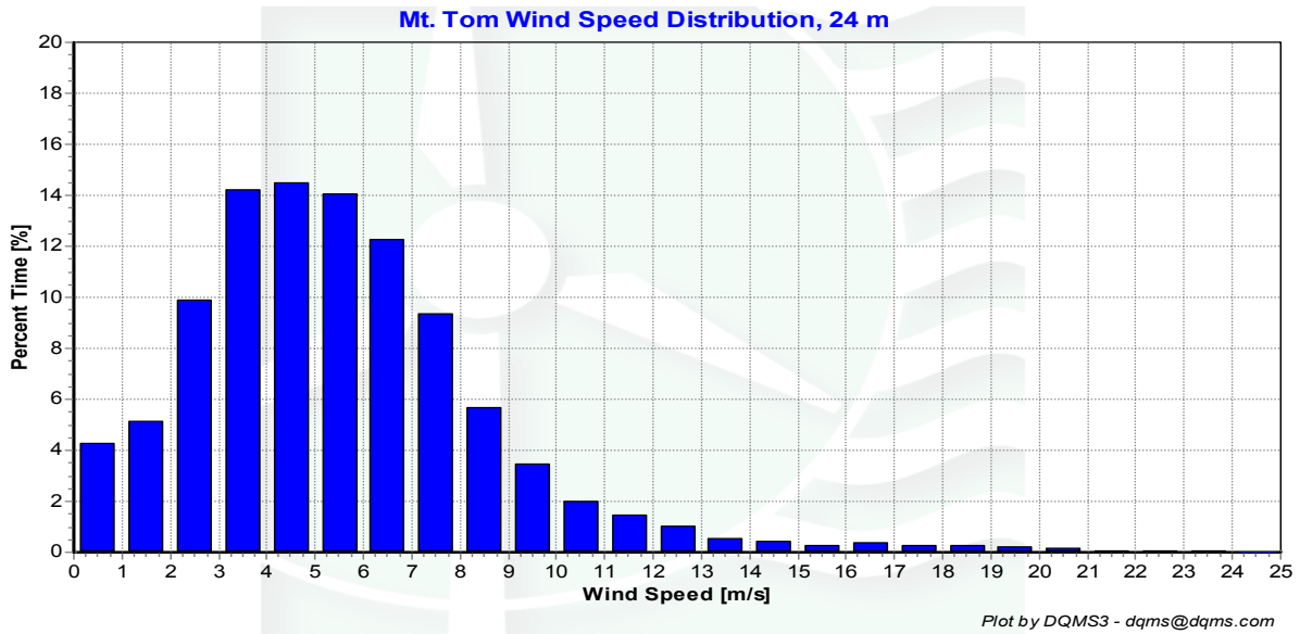
Figure 3 - Wind Speed Distribution, September 2003 – November 2003
