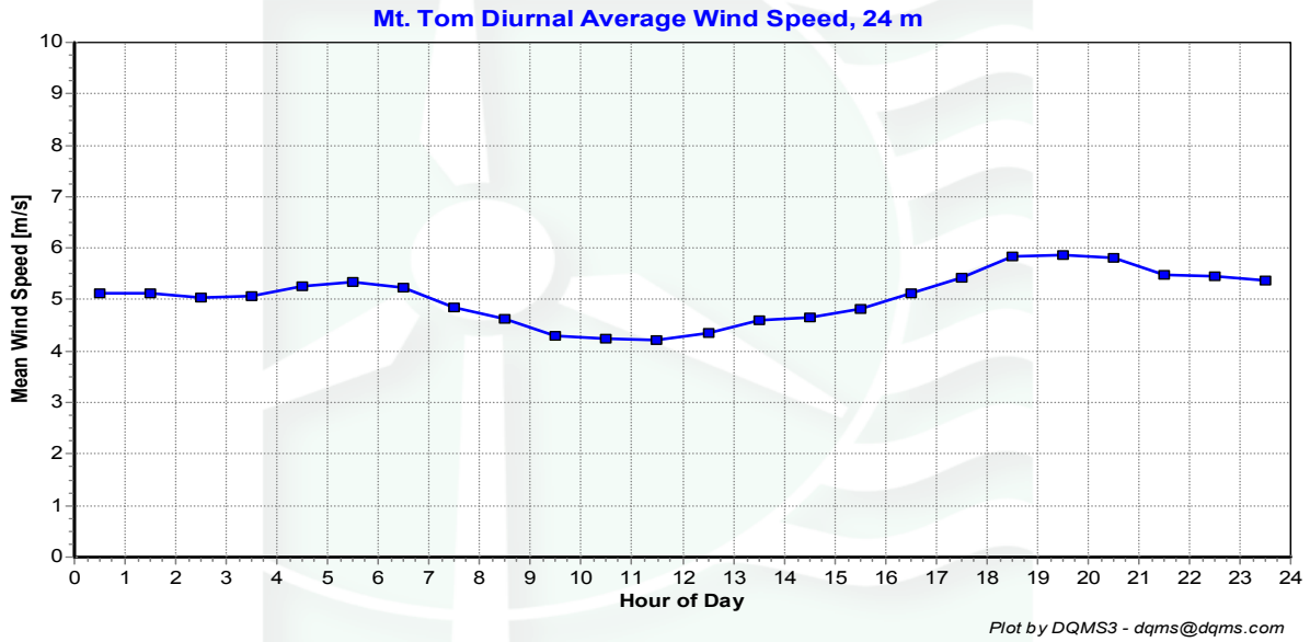
Figure 5 - Diurnal Wind Speed, September 2003 – November 2003
