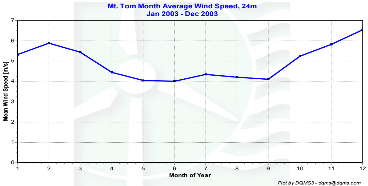
Figure 4 - Monthly average wind speed
