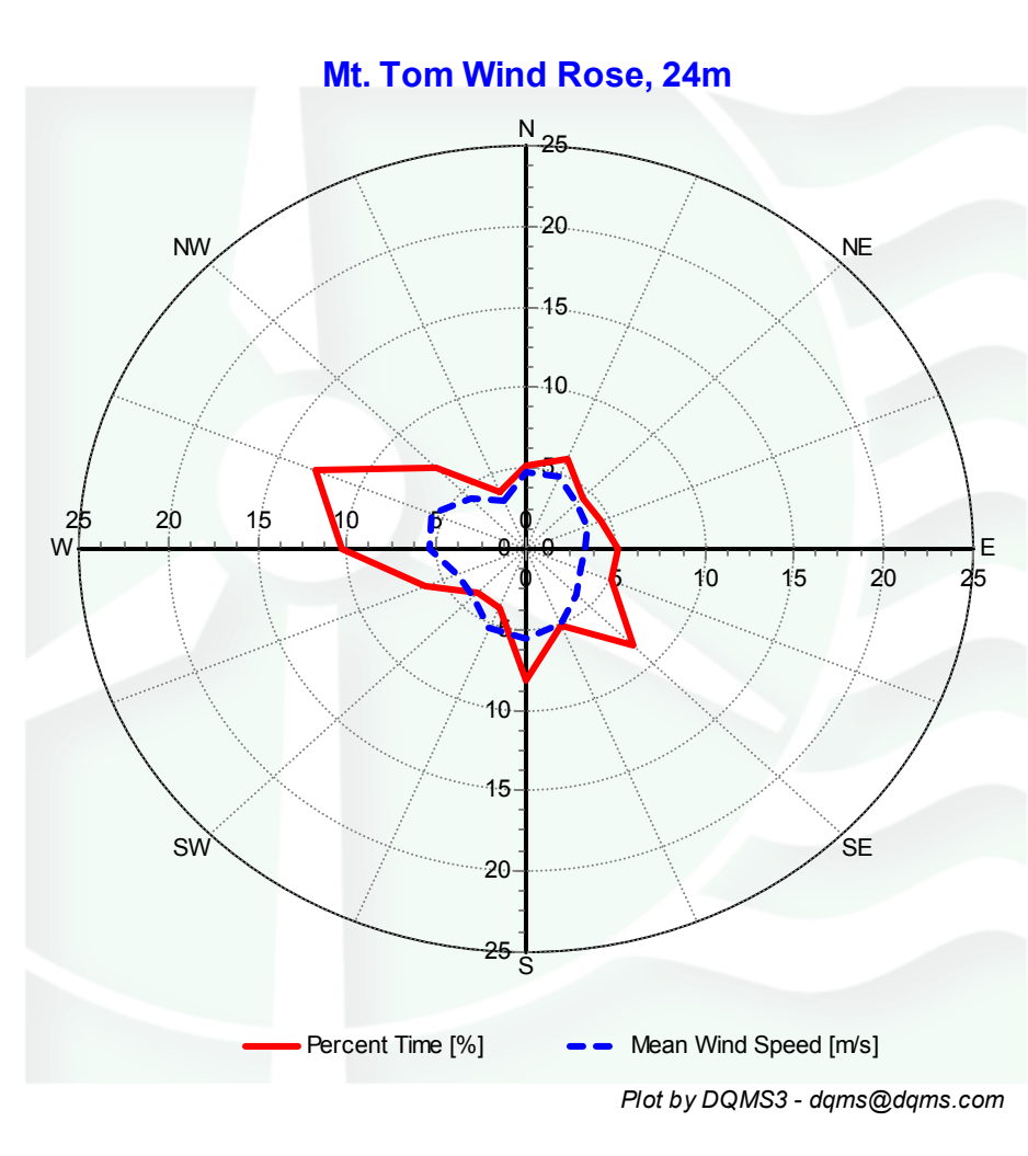
Figure 7 - Wind Rose, September 2003 – November 2003
