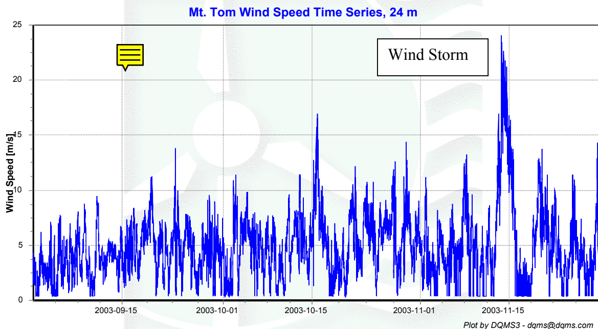
Figure 2 - Wind Speed Time Series, September 2003 – November 2003
