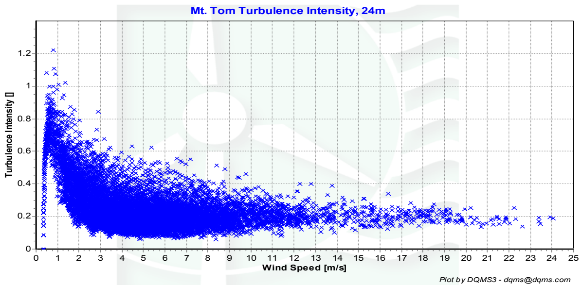
Figure 6 - Turbulence Intensity vs. Wind Speed, September 2003 – November 2003
