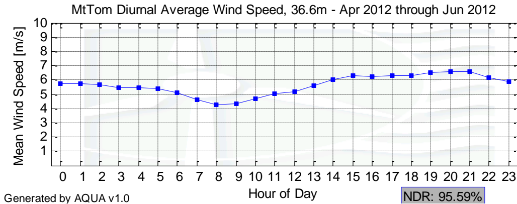
Figure 5 - Mt. Tom Diurnal Average Wind Speed, 36.6 m, April 1 – June 30, 2012
