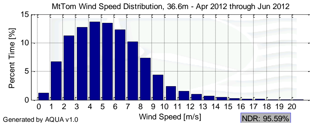
Figure 3 - Mt. Tom Wind Speed Distributions, April 1 – June 30, 2012
