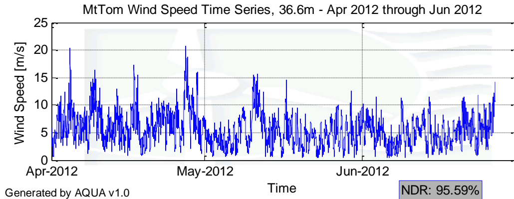
Figure 2 – Mt. Tom Wind Speed Time Series, 36.6 m, April 1 – June 30, 2012
