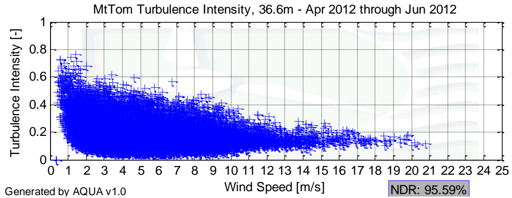
Figure 6 - Mt. Tom Turbulence Intensity, 36.6 m, April 1 – June 30, 2012
