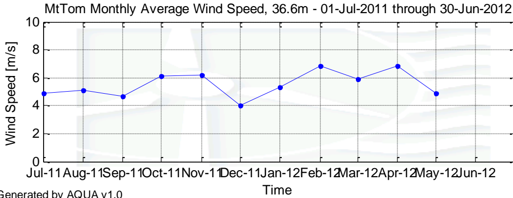
Figure 4 – Mt. Tom Monthly Average Wind Speeds, July 1, 2011 –June 30, 2012
