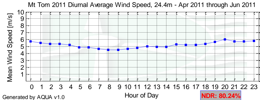
Figure 5 - Mt. Tom Diurnal Average Wind Speed, 24.4 m, April 1 – June 30, 2011
