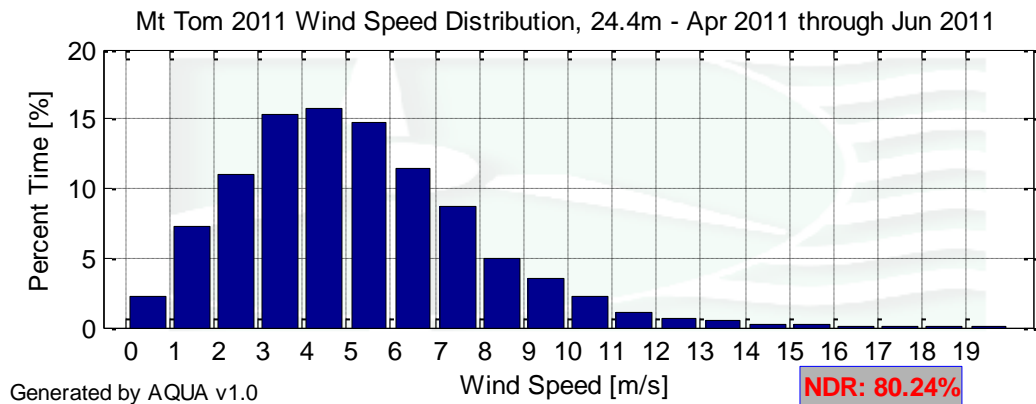
Figure 3 - Mt. Tom Wind Speed Distributions, 24.4 m, April 1 – June 30, 2011
