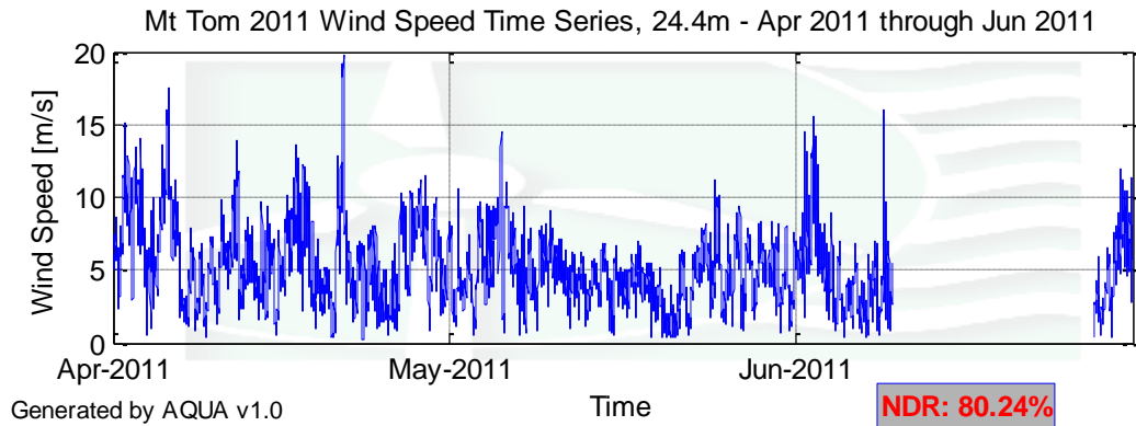
Figure 2 – Mt. Tom Wind Speed Time Series, 24.4 m, April 1 – June 30, 2011
