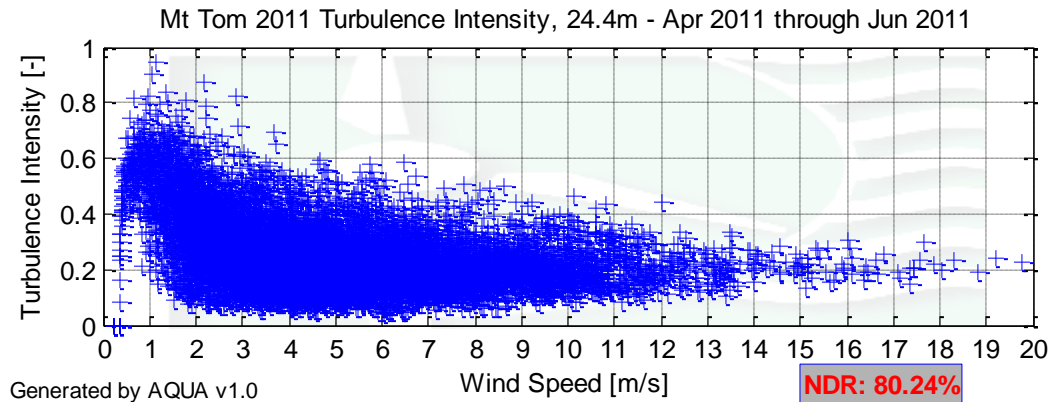
Figure 6 - Mt. Tom Turbulence Intensity, 24.4 m, April 1 – June 30, 2011
