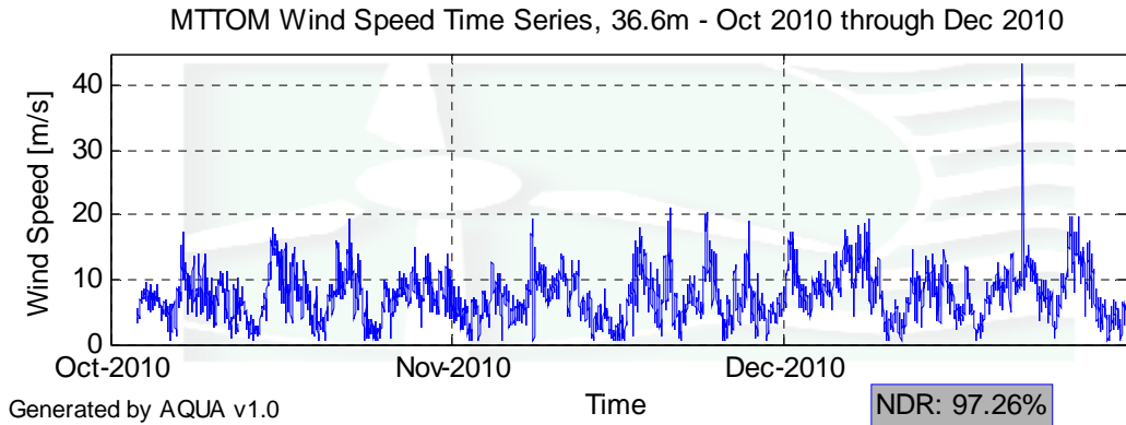
Figure 2 – Mt. Tom Wind Speed Time Series, 36.6 m, October 1 – December 31, 2010
