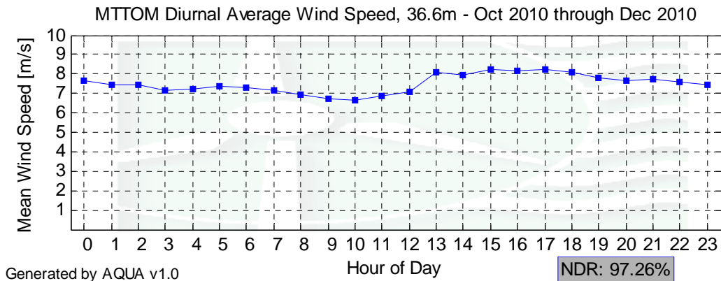
Figure 5 - Mt. Tom Diurnal Average Wind Speed, 36.6 m, October 1 – December 31, 2010
