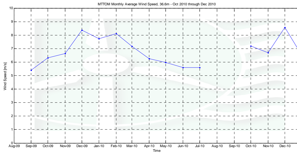
Figure 4 – Mt. Tom Monthly Average Wind Speeds, October 1 – December 31, 2010
