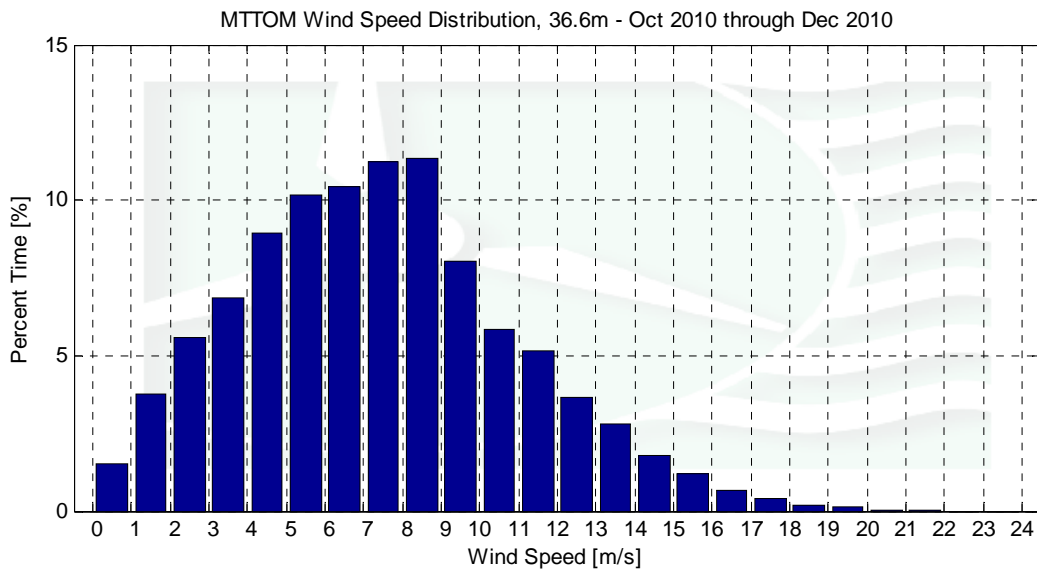
Figure 3 - Mt. Tom Wind Speed Distributions, 36.6 m, October 1 – December 31, 2010
