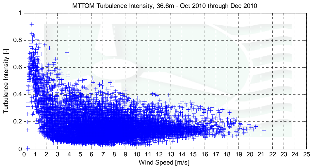
Figure 6 - Mt. Tom Turbulence Intensity, 36.6 m, October 1 – December 31, 2010
