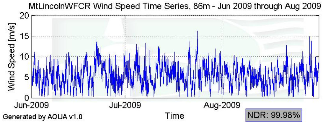
Figure 2 – Wind Speed Time Series, June 1, 2009 – August 31, 2009
