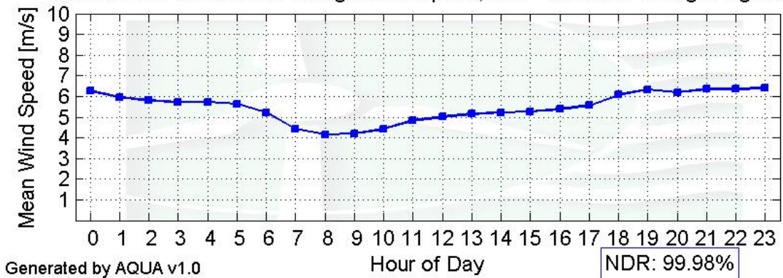
Figure 5 – Diurnal Average Wind Speeds, June 1, 2009 – August 31, 2009
