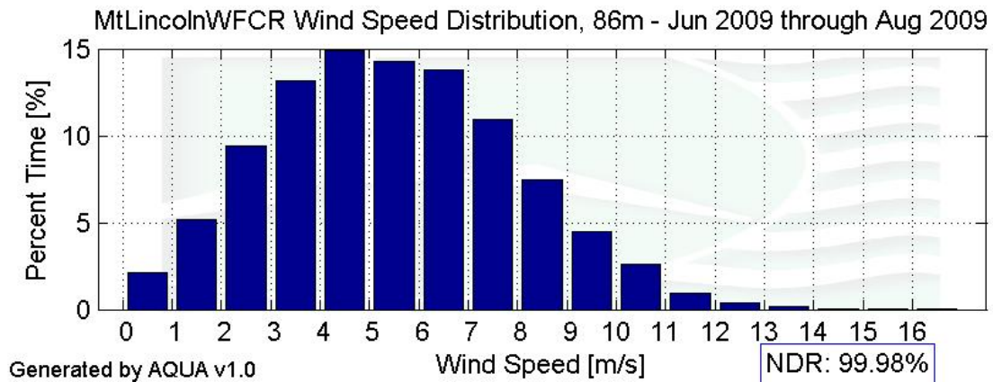
Figure 3 – Wind Speed Distribution, June 1, 2009 – August 31, 2009
