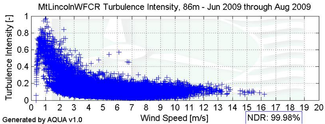
Figure 6 – Turbulence Intensity vs. Wind Speed, June 1, 2009 – August 31, 2009
