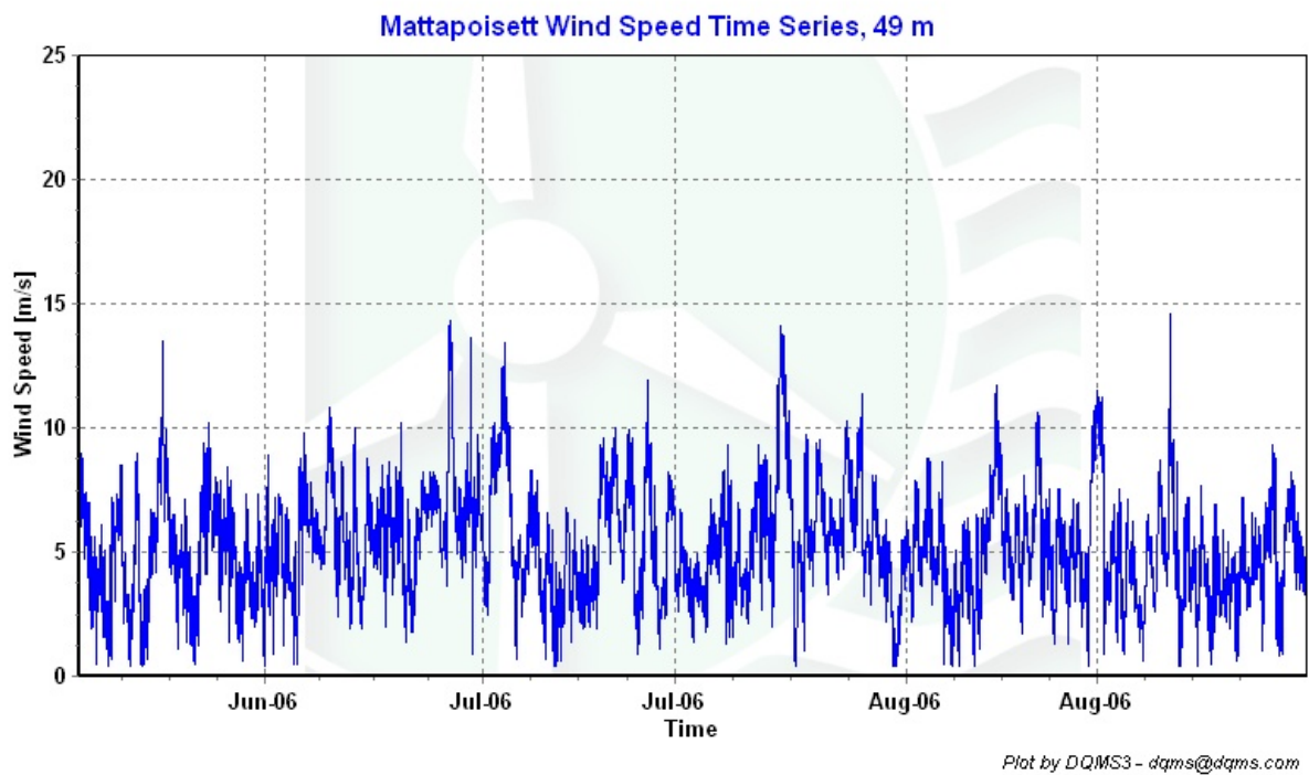
Figure 2 – Wind Speed Time Series, June 1, 2006 through August 31, 2006
