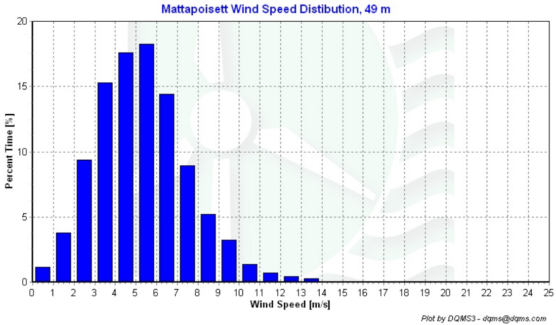
Figure 3 – Wind Speed Distribution, June 1, 2006 through August 31, 2006
