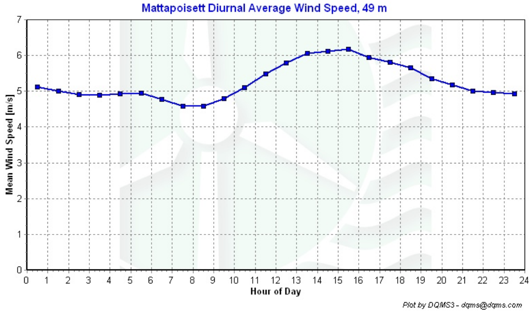
Figure 5 – Diurnal Average Wind Speed, June 1, 2006 through August 31, 2006
