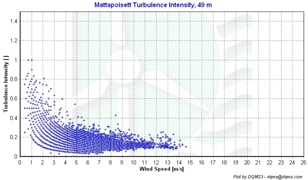
Figure 6 – Turbulence Intensity, June 1, 2006 through August 31, 2006
