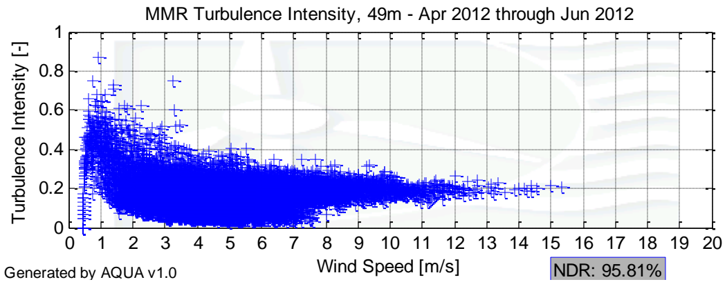
Figure 6 – MMR Turbulence Intensity for April 1 to June 30, 2012
