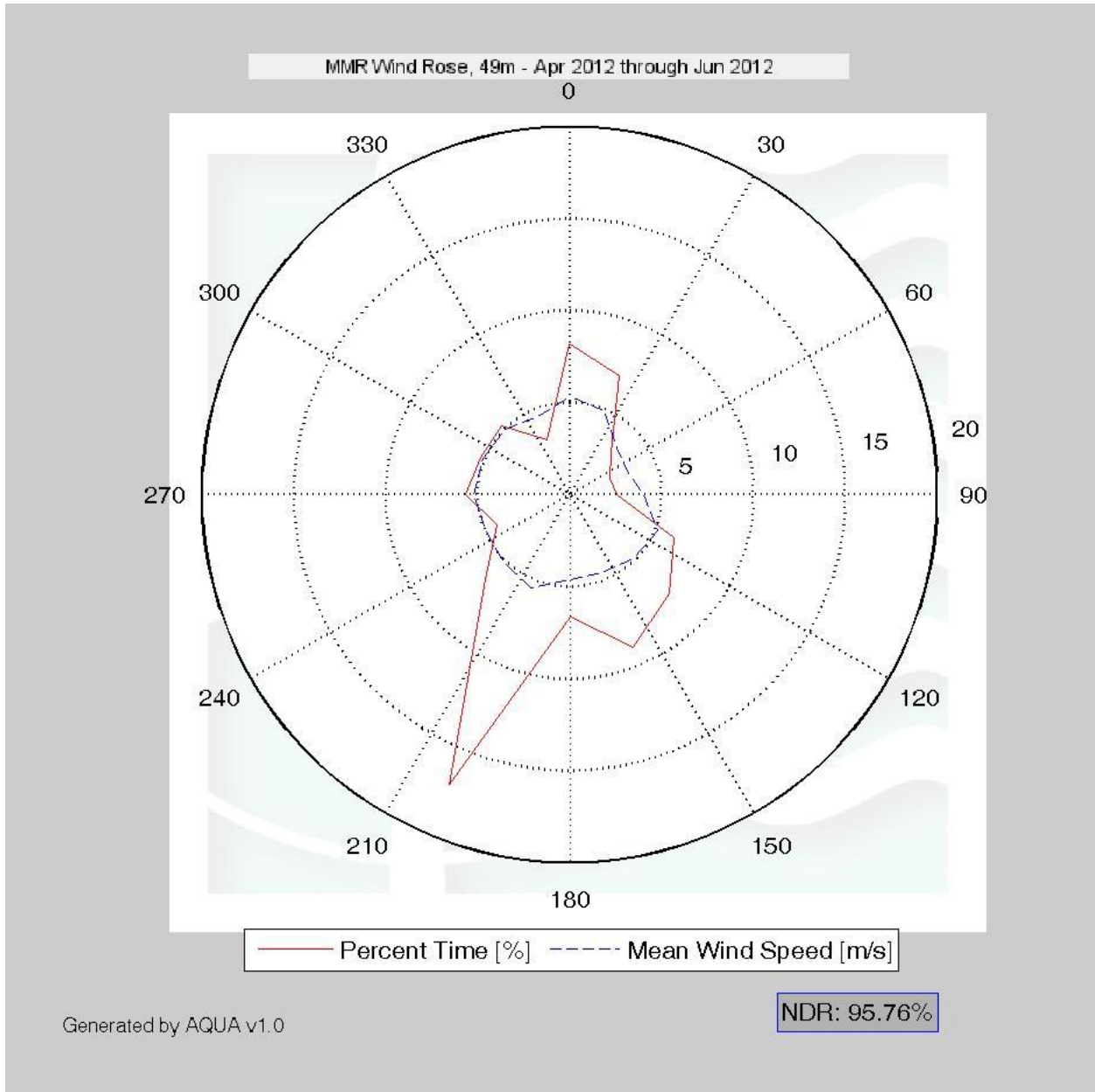
Figure 7 – MMR Wind Rose for April 1 to June 30, 2012
