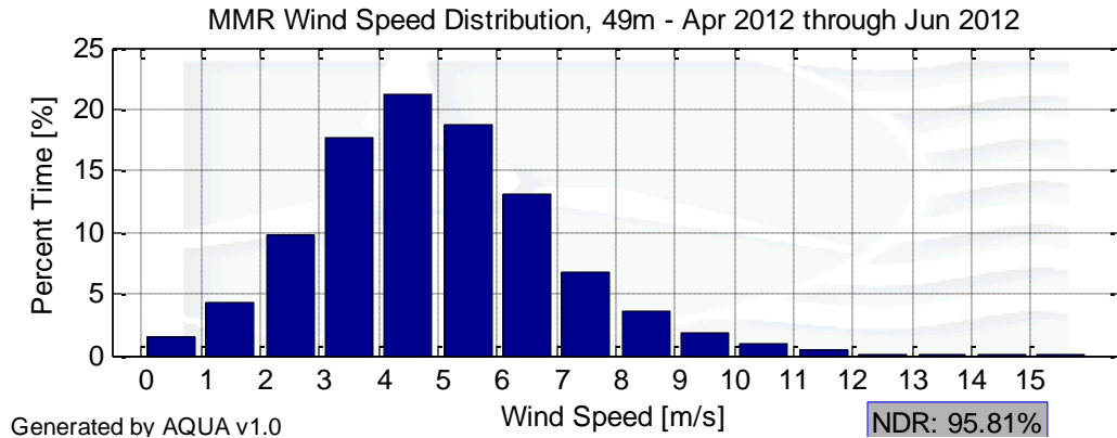
Figure 3 – MMR Wind Speed Distribution April 1 to June 30, 2012
