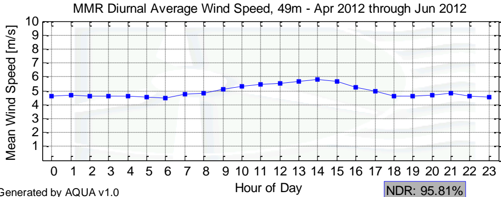
Figure 5 – MMR Diurnal Average Wind Speeds for April 1 to June 30, 2012
