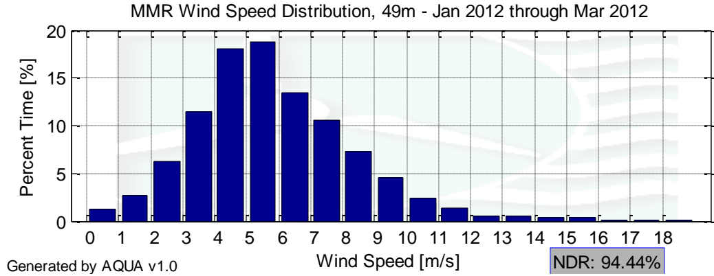
Figure 3 – MMR Wind Speed Distribution January 1 to March 31, 2012
