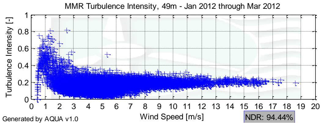
Figure 6 – MMR Turbulence Intensity for January 1 March 31, 2012
