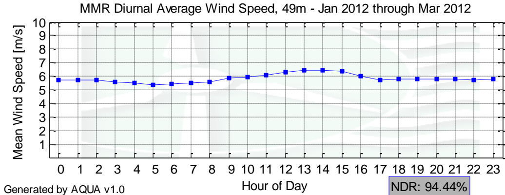
Figure 5 – MMR Diurnal Average Wind Speeds for January 1 March 31, 2012
