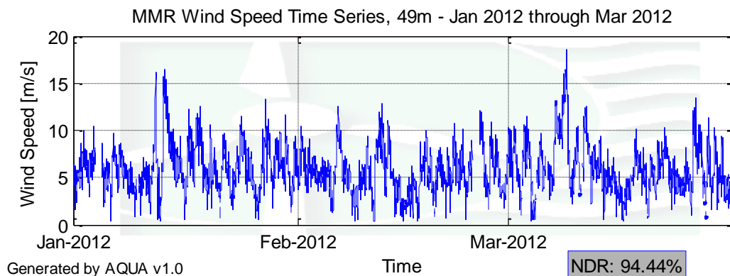
Figure 2 – MMR Wind Speed Time Series for January 1 to March 31, 2012
