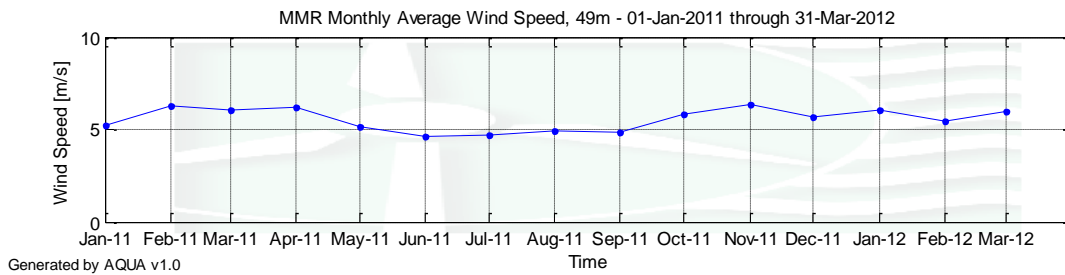
Figure 4 – MMR Monthly Wind Speed Averages for January 1, 2010 to March 31, 2012
