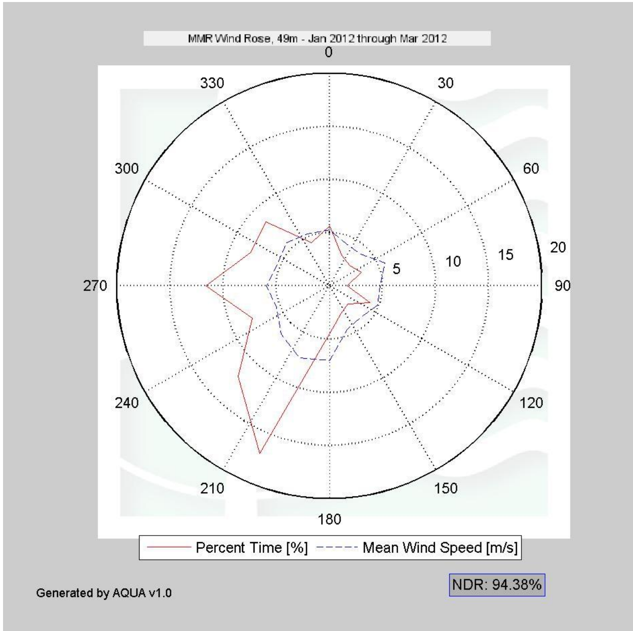
Figure 7 – MMR Wind Rose for January 1 to March 31, 2012
