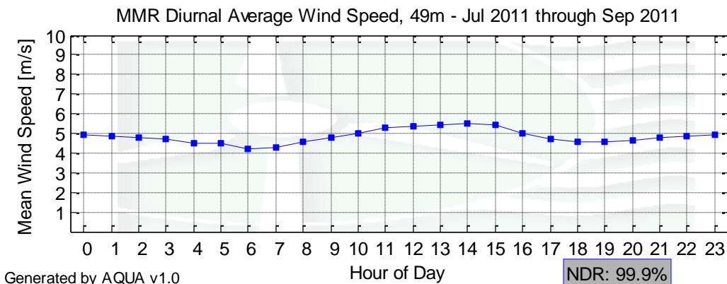
Figure 5 – Diurnal Average Wind Speeds for July 1 to September 30, 2011
