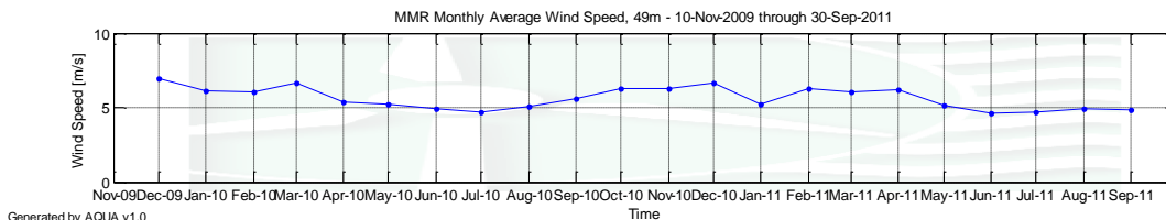
Figure 4 – MMR Monthly Wind Speed Averages for December 1 2009 to September 30 2011
