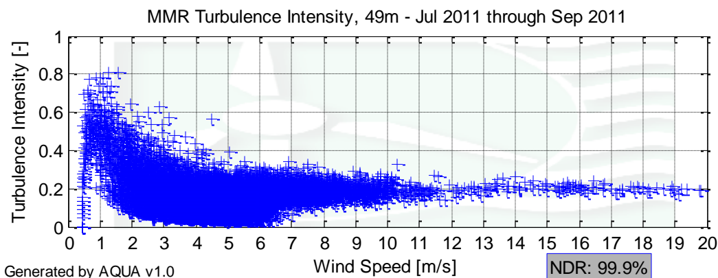
Figure 6 – Turbulence Intensity for July 1 to September 30, 2011
