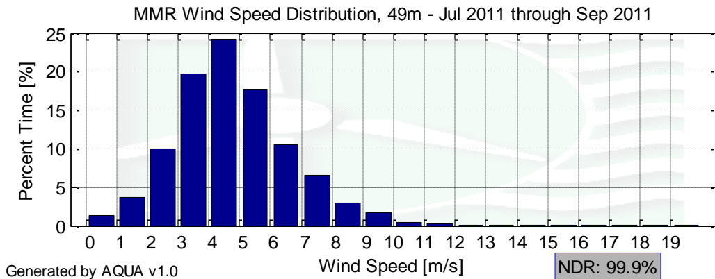
Figure 3 – MMR Wind Speed Distribution for July 1 to September 30, 2011
