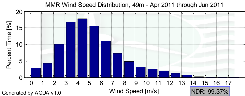
Figure 3 – MMR Wind Speed Distribution for April 1 to June 30, 2011
