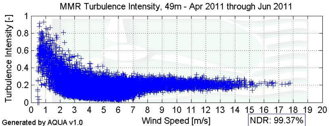
Figure 6 – Turbulence Intensity for April 1 to June 30, 2011
