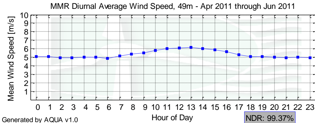
Figure 5 – Diurnal Average Wind Speeds for April 1 to June 30, 2011
