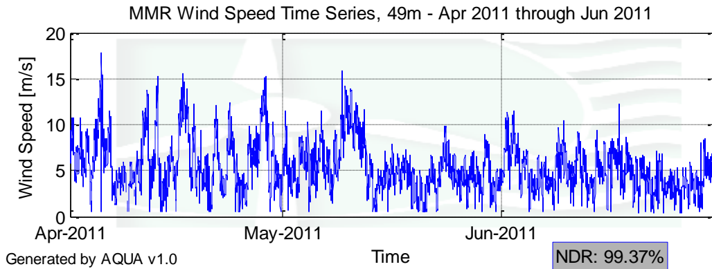
Figure 2 – MMR Wind Speed Time Series for April 1 to June 30, 2011
