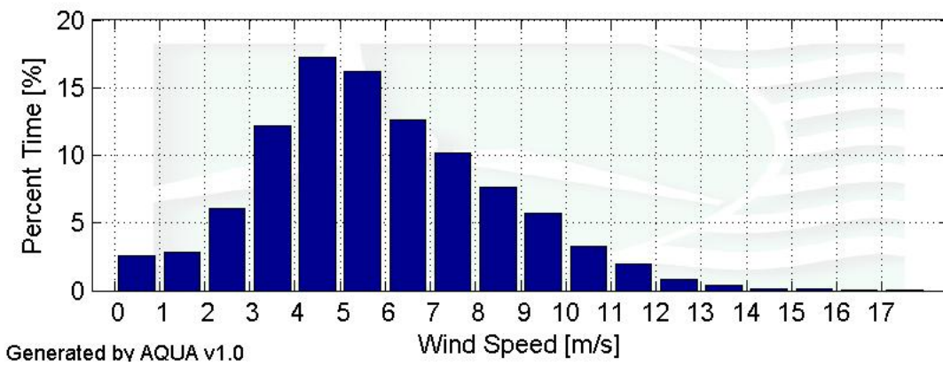
Figure 3 – MMR Wind Speed Distribution for January 1 to March 31, 2011
