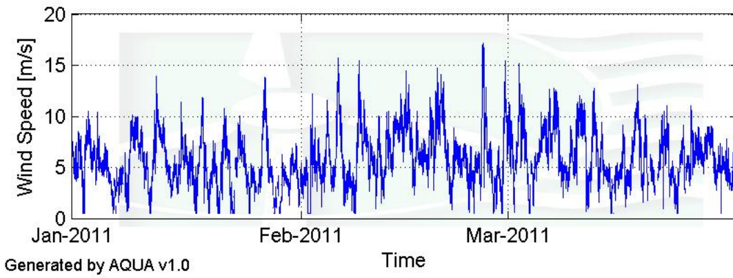
Figure 2 – MMR Wind Speed Time Series for January 1 to March 31, 2011
