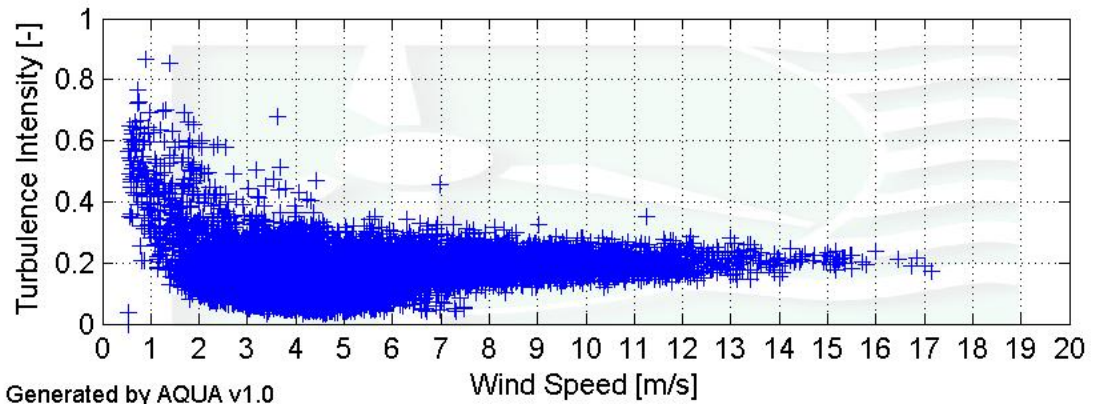
Figure 6 – Turbulence Intensity for January 1 to March 31, 2011
