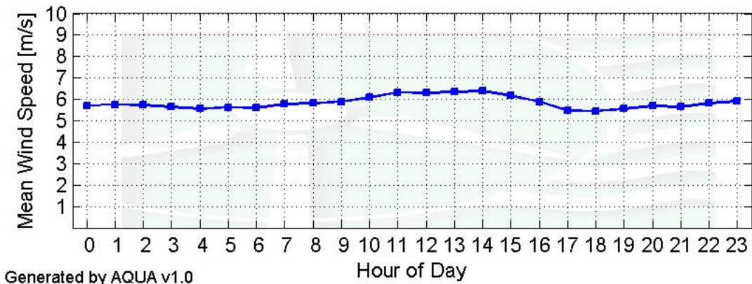
Figure 5 – Diurnal Average Wind Speeds for January 1 to March 31, 2011
