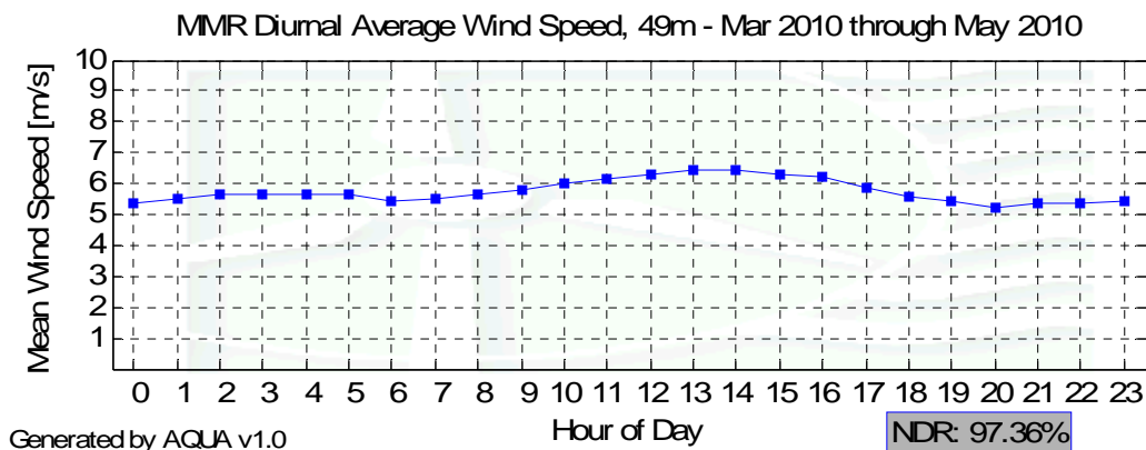
Figure 5 – Diurnal Average Wind Speeds for March 1 to May 31
