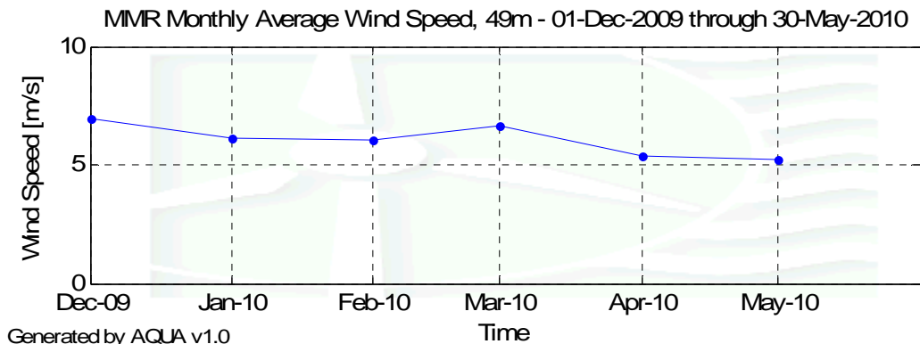
Figure 4 – MMR Monthly Wind Speed Averages for December 1 to May 31
