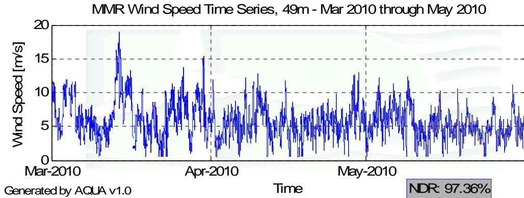
Figure 2 – MMR Wind Speed Time Series for March 1 to May 31
