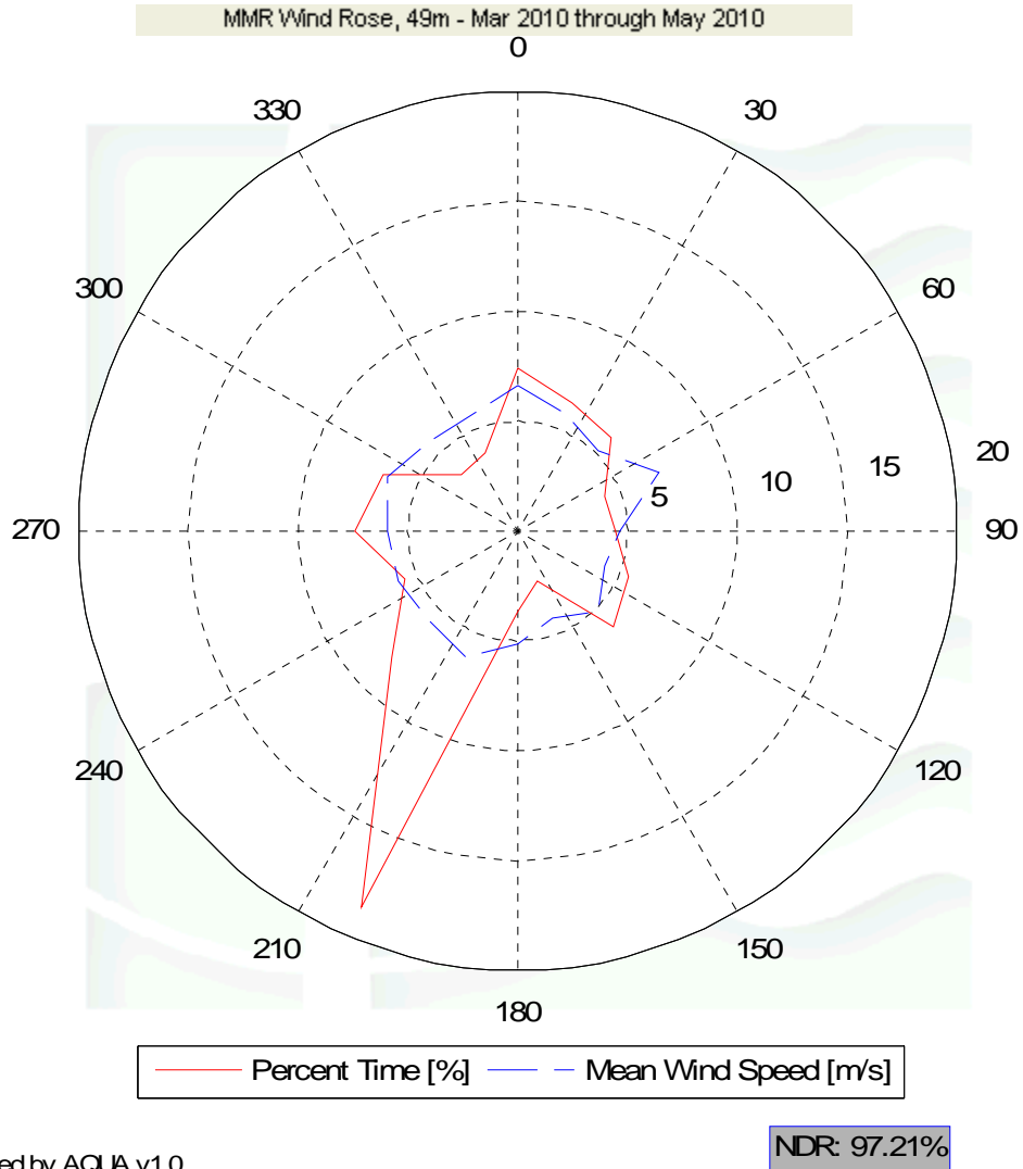
Figure 7 – Wind Rose for March 1 to May 31
