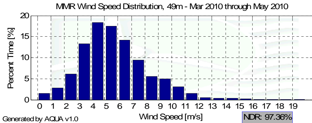
Figure 3 – MMR Wind Speed Distribution for March 1 to May 31
