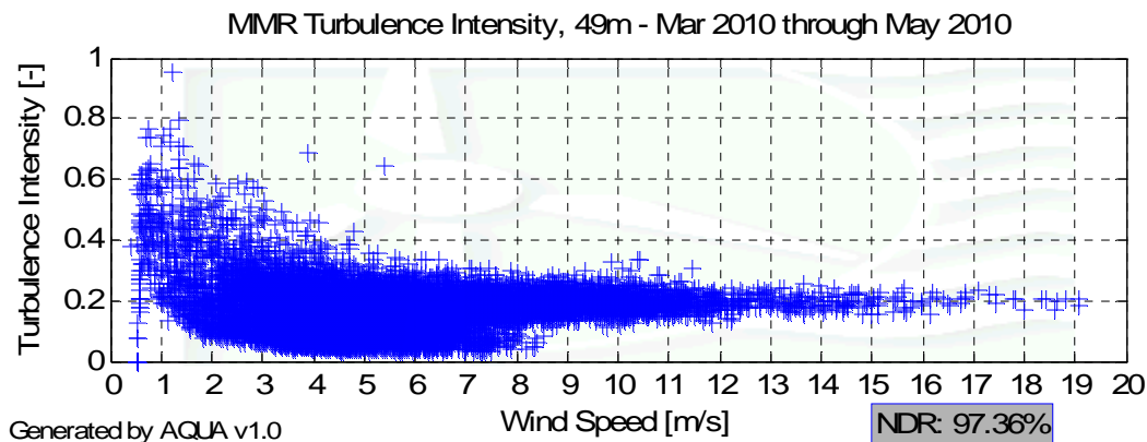
Figure 6 – Turbulence Intensity for March 1 to May 31
