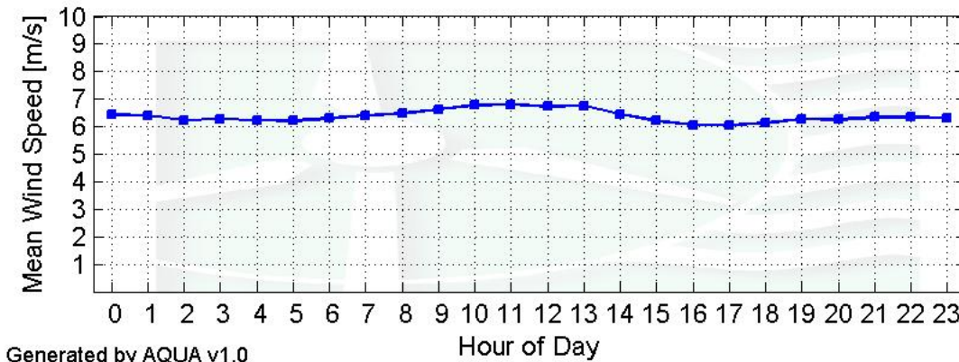
Figure 5 – Diurnal Average Wind Speeds for October 1 to December 31
