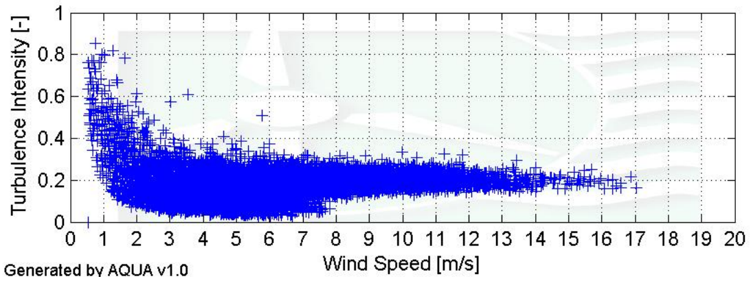
Figure 6 – Turbulence Intensity for October 1 to December 31
