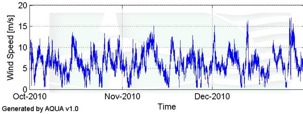
Figure 2 – MMR Wind Speed Time Series for October 1 to December 31
