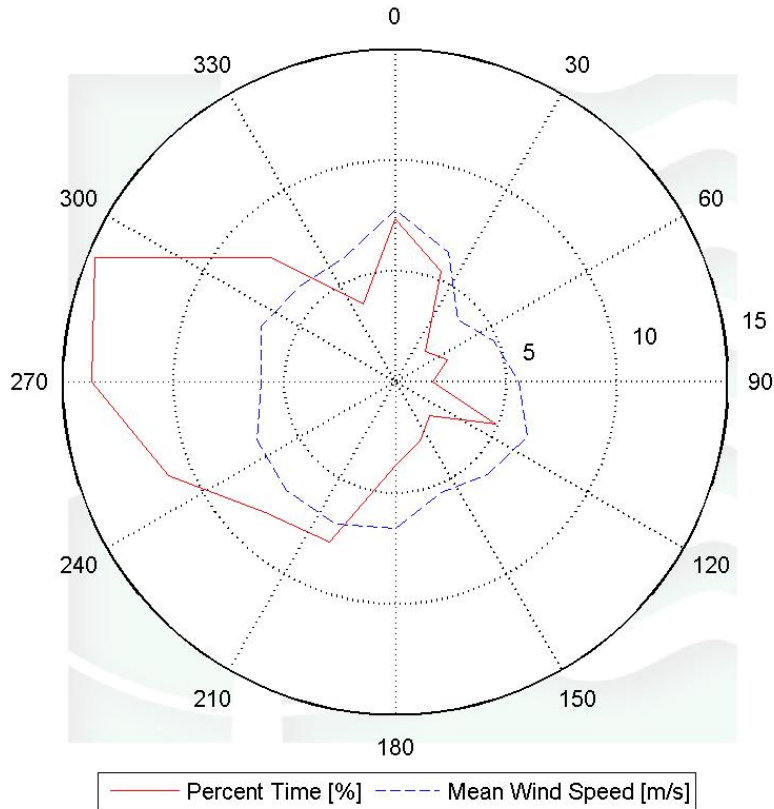
Figure 7 – Wind Rose for October 1 to December 31
