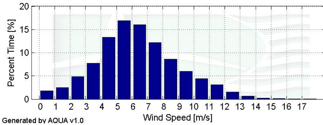
Figure 3 – MMR Wind Speed Distribution for October 1 to December 31
