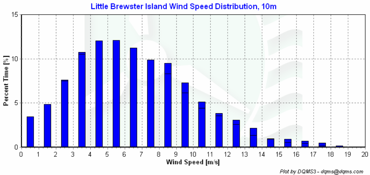
Figure 3 - Little Brewster Island Wind Speed Distribution March 1 st , 2008 to May 31 st , 2008
