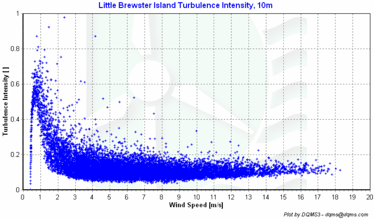
Figure 6 - Little Brewster Island Turbulence Intensity March 1 st , 2008 to May 31 st , 2008
