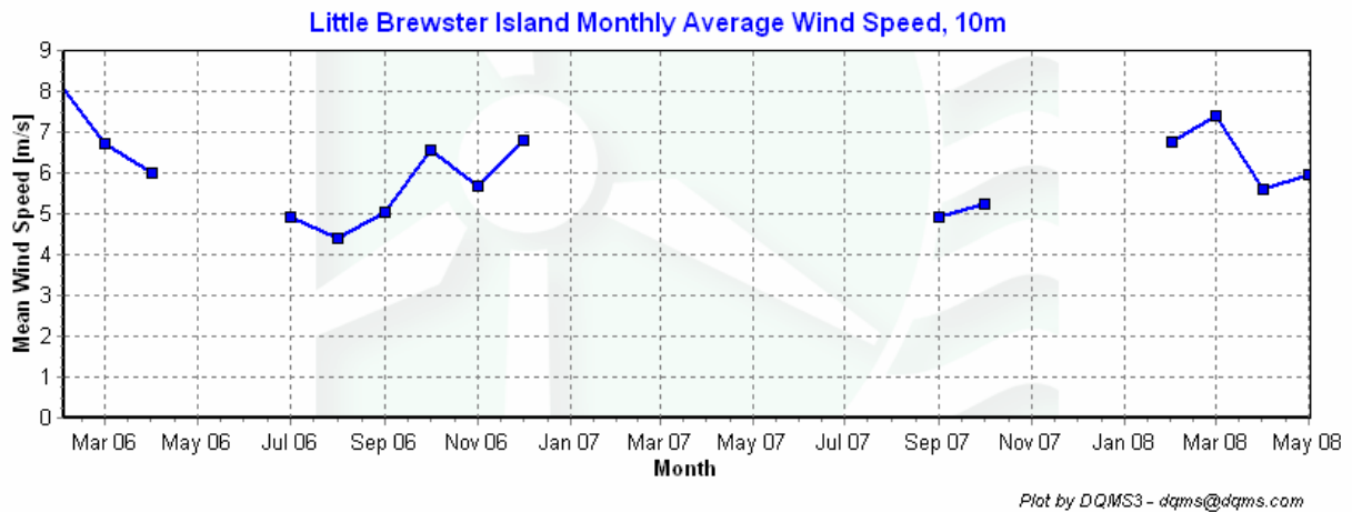
Figure 4 - Little Brewster Island Monthly Average Wind Speed Feb 2006 – May 2008
