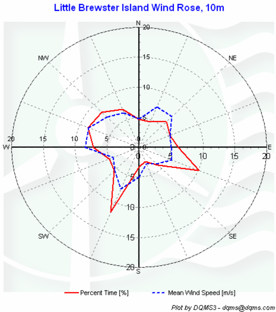
Figure 7 - Little Brewster Island Wind Rose March 1 st , 2008 to May 31 st , 2008
