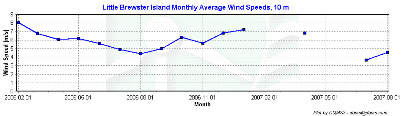
Figure 4 - Little Brewster Island Monthly Average Wind Speed Feb 2006 – Aug 2007
