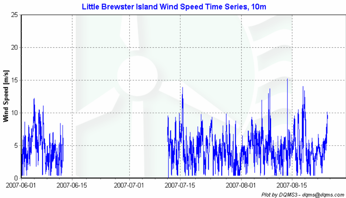
Figure 2 - Little Brewster Island Wind Speed Time Series June 1 st , 2007 to August 31 st , 2007
