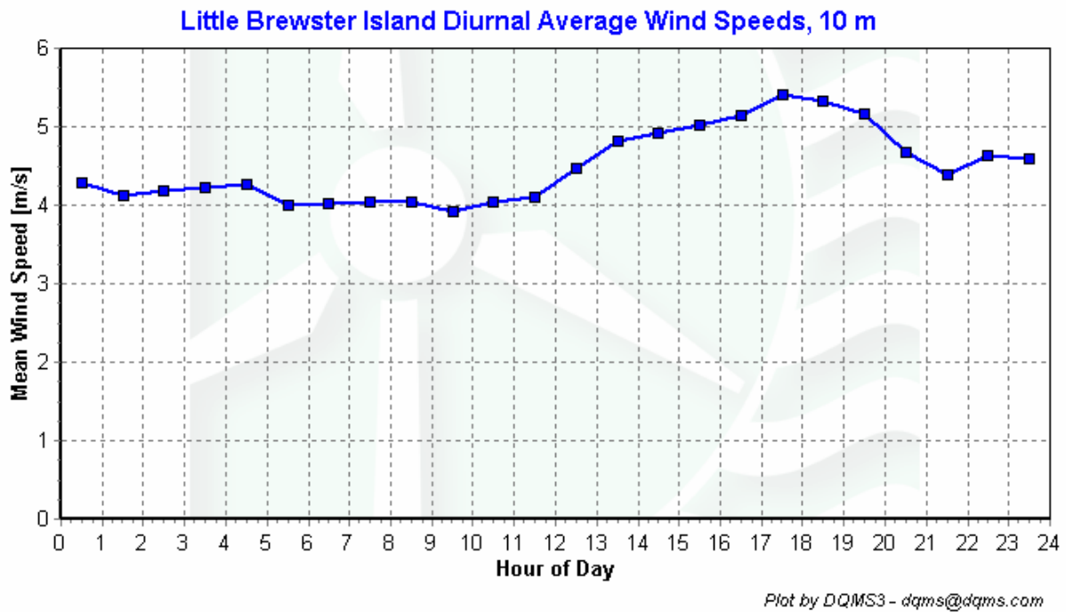
Figure 5 - Little Brewster Island Diurnal Average Wind Speed June 1 st , 2007 to August 31 st , 2007
