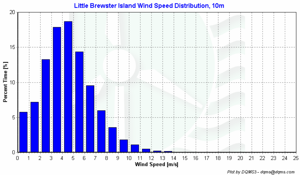
Figure 3 - Little Brewster Island Wind Speed Distribution June 1 st , 2007 to August 31 st , 2007
