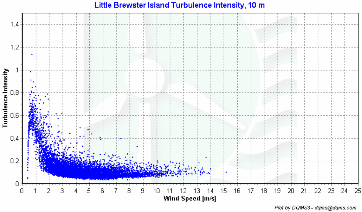
Figure 6 - Little Brewster Island Turbulence Intensity June 1 st , 2007 to August 31 st , 2007
