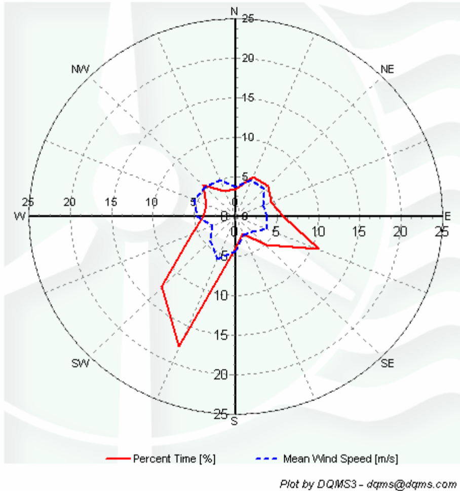
Little Brewster Island Wind Rose, 10m
