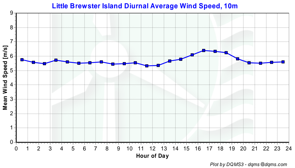
Figure 5 - Little Brewster Island Diurnal Average Wind Speed September 1 st , 2007 to November 30 th , 2007
