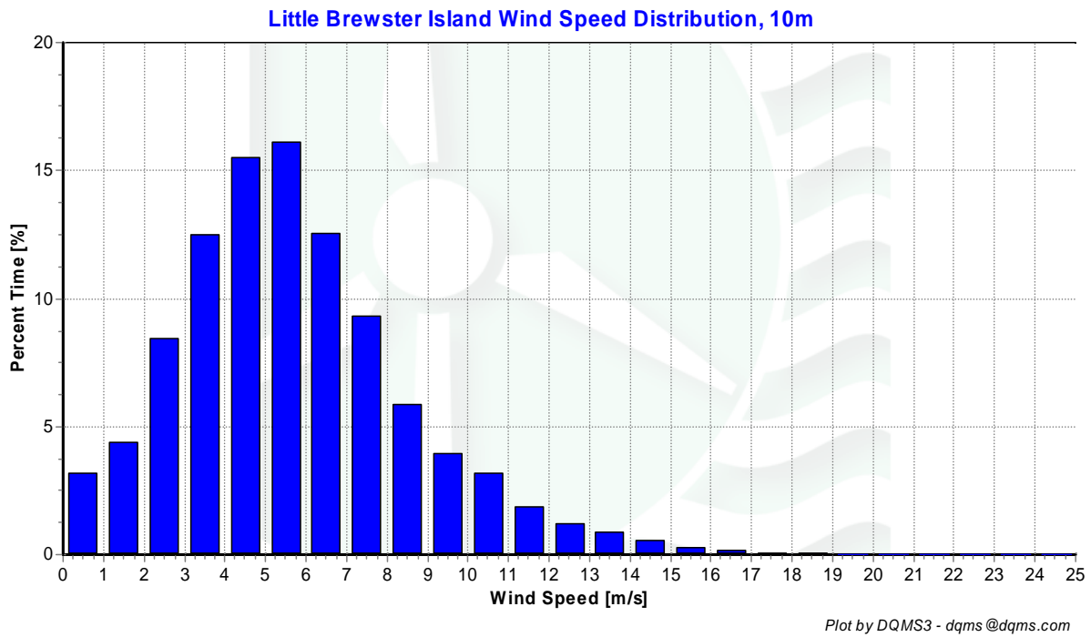
Figure 3 - Little Brewster Island Wind Speed Distribution September 1 st , 2007 to November 30 th , 2007
