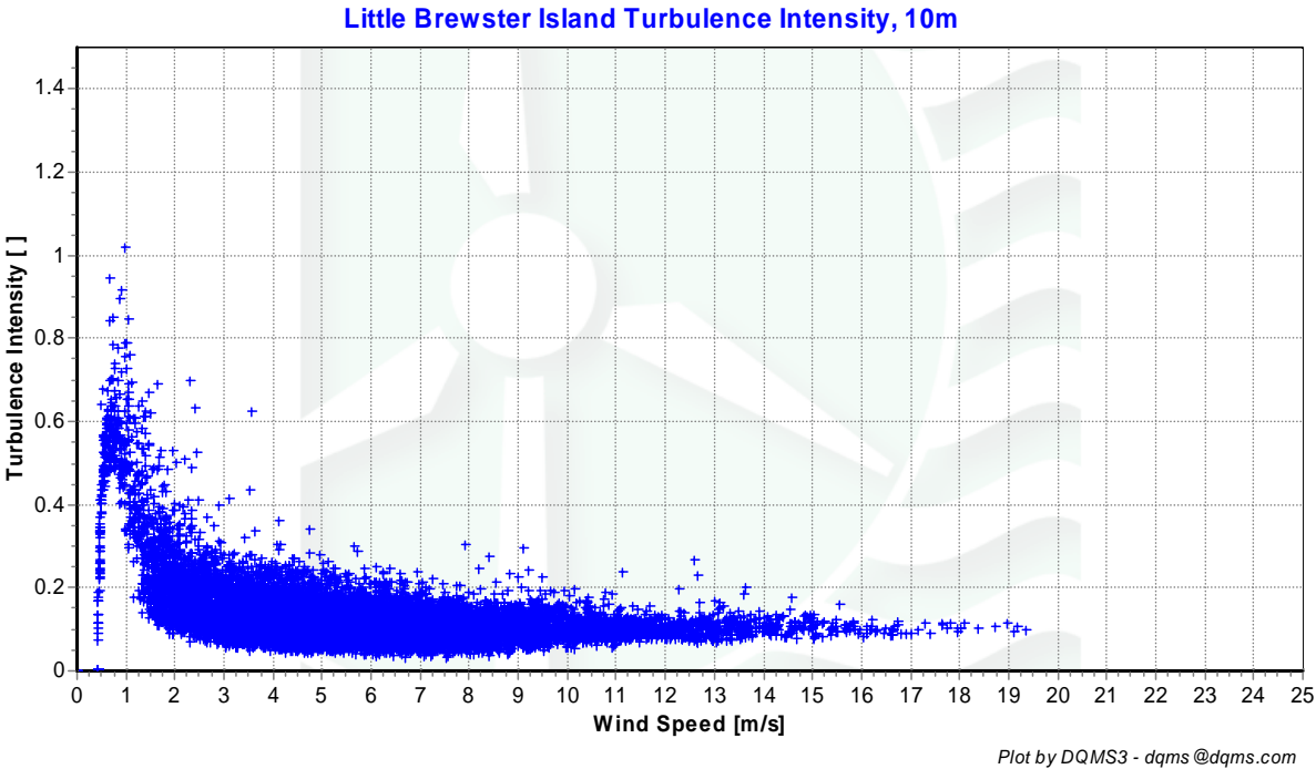
Figure 6 - Little Brewster Island Turbulence Intensity September 1 st , 2007 to November 30 th , 2007
