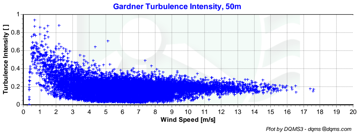
Figure 6 – Turbulent Intensity vs. Wind Speed, March 1, 2007 – May 31, 2007
