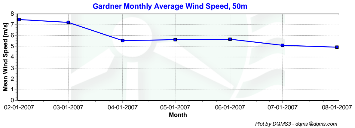
Figure 4 – Monthly Average Wind Speeds, February 1, 2007 – August 31, 2007
