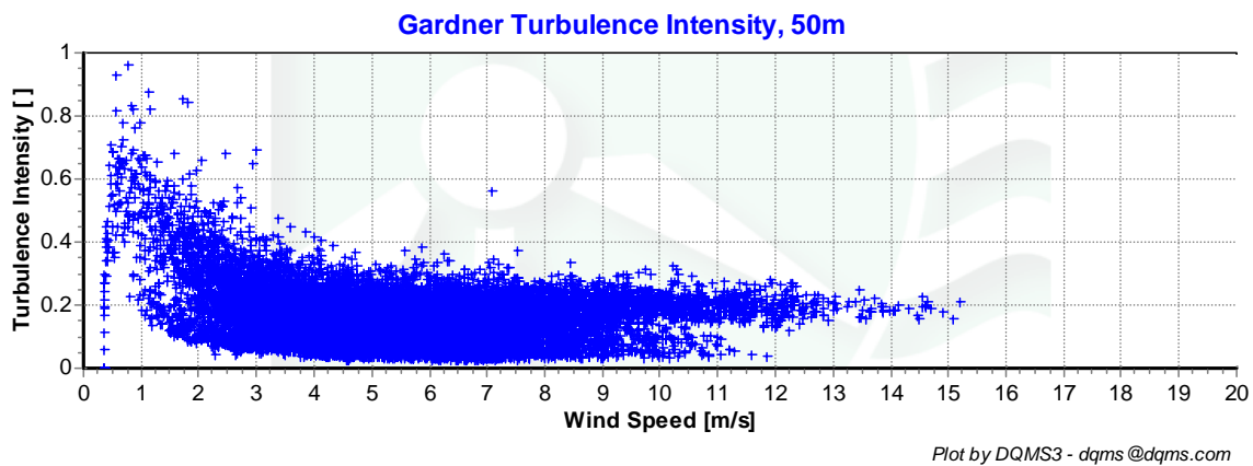
Figure 6 – Turbulent Intensity vs. Wind Speed, September 1, 2007 – November 30, 2007
