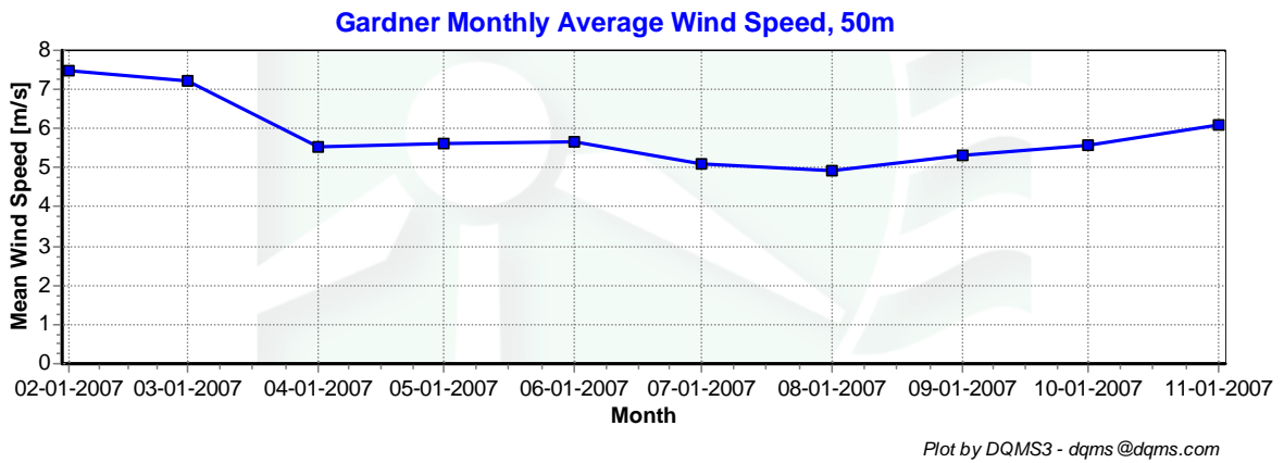
Figure 4 – Monthly Average Wind Speeds, February 1, 2007 – November 30, 2007
