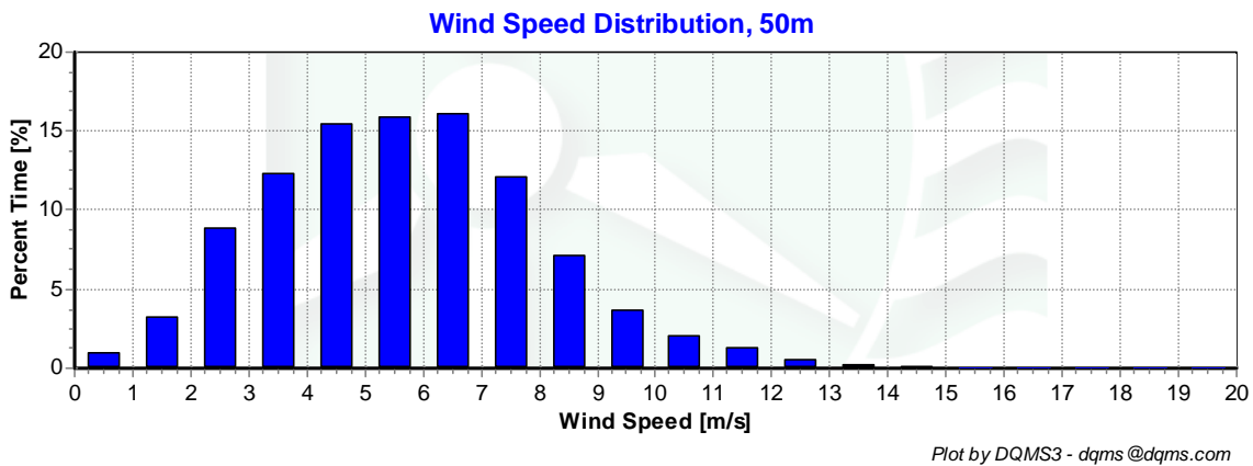
Figure 3 – Wind Speed Distribution, September 1, 2007 – November 30, 2007
