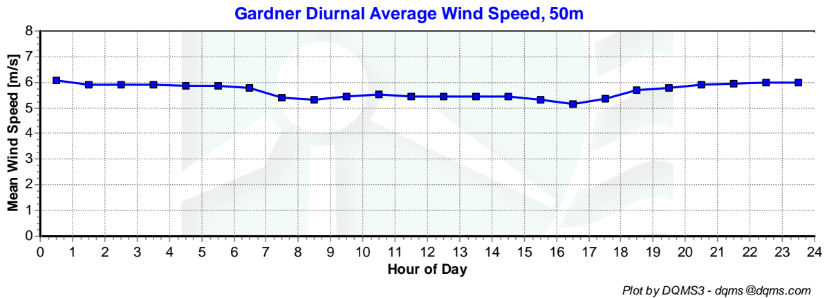
Figure 5 – Diurnal Average Wind Speed, September 1, 2007 – November 30, 2007
