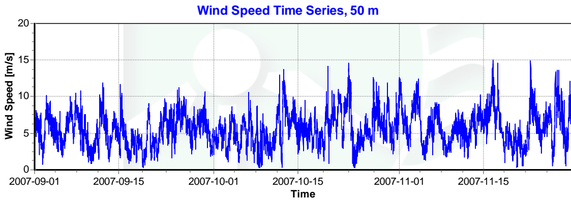
Figure 2 – Wind Speed Time Series, September 1, 2007 – November 30, 2007
