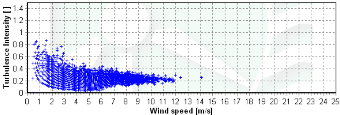
Figure 6 - Turbulence Intensity vs. Wind Speed, March 1, 2006 – May 31, 2006.
