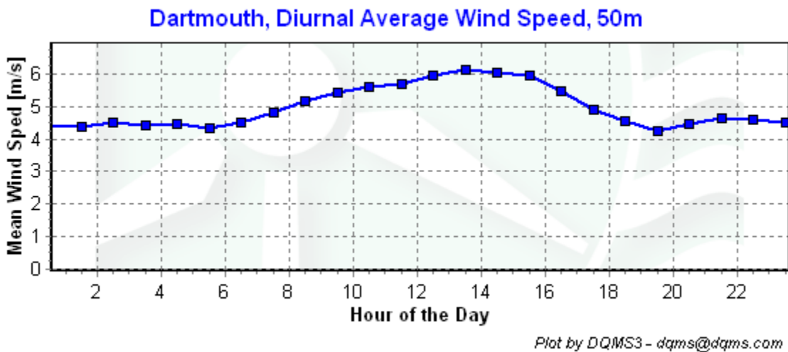
Figure 5 - Diurnal Wind Speed, March 1, 2006 – May 31, 2006.
