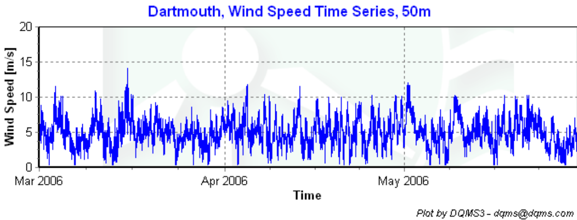
Figure 2 - Wind Speed Time Series, March 1, 2006 – May 31, 2006.
